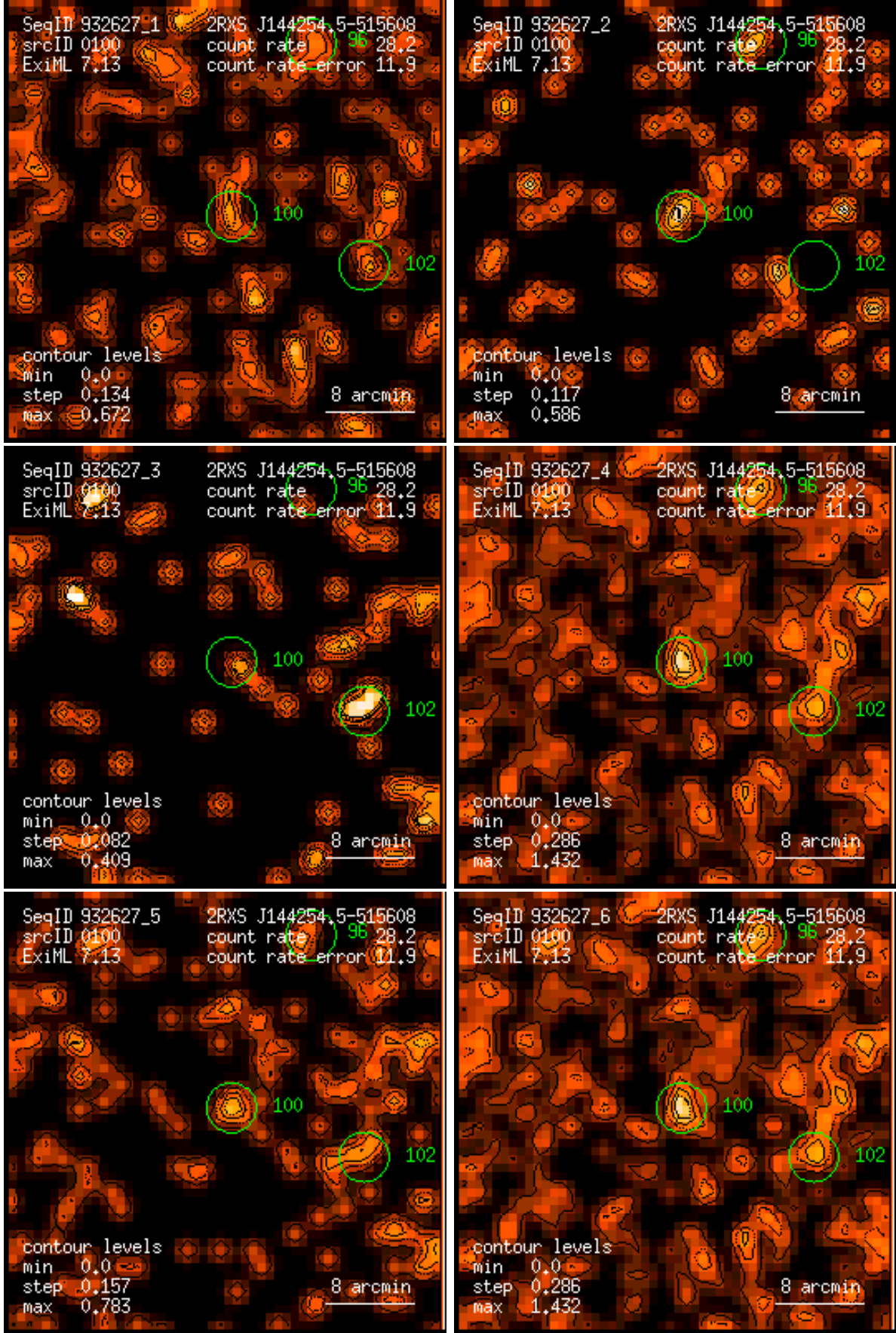
Figure 100: RASS 932627: detection 0100: band rate images, Gaussian filter: (1) PSPC channels 11 – 41, (2) 52 – 90, (3) 91 – 201, (4) 11 – 235, (5) 52 – 201, (6) 11 – 201. Broad band rates in counts/ks. Band rate contour levels in counts/ks/arcmin 2 .
