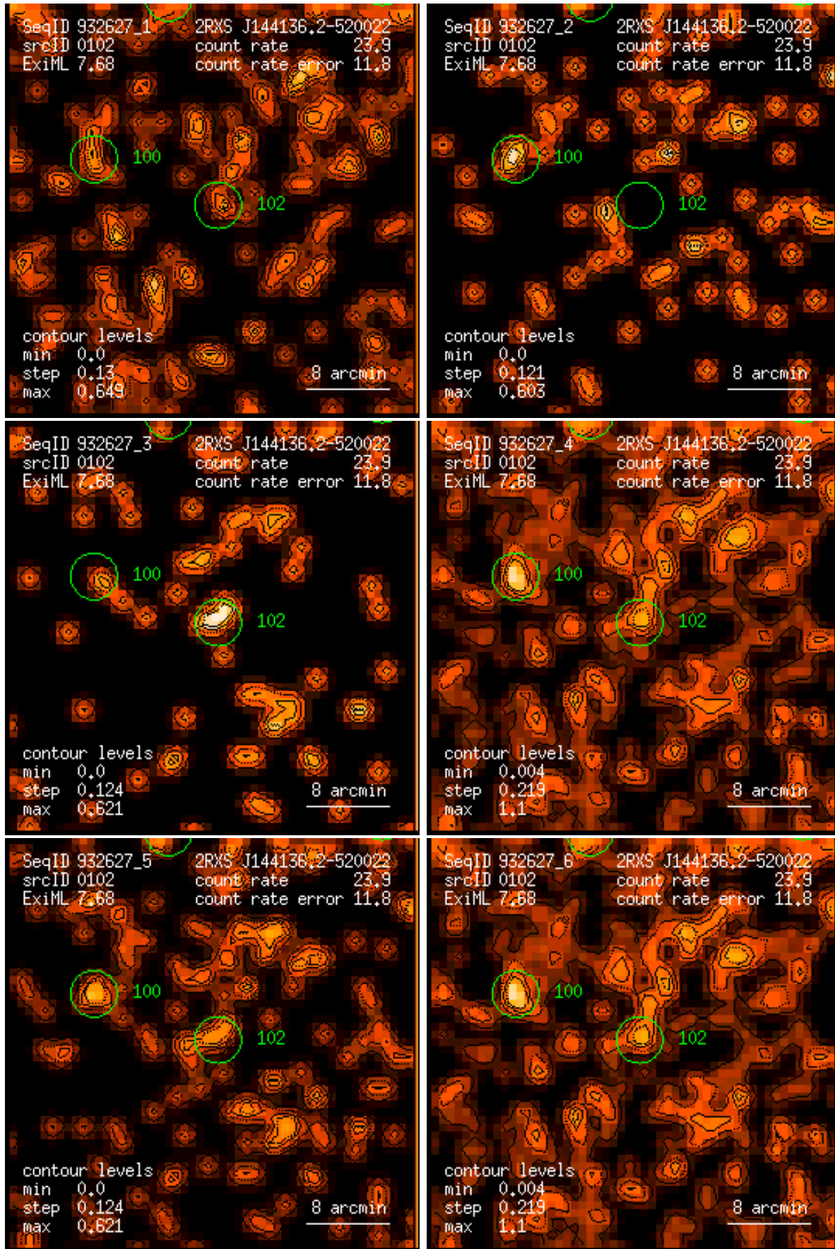
Figure 102: RASS 932627: detection 0102: band rate images, Gaussian filter: (1) PSPC channels 11 – 41, (2) 52 – 90, (3) 91 – 201, (4) 11 – 235, (5) 52 – 201, (6) 11 – 201. Broad band rates in counts/ks. Band rate contour levels in counts/ks/arcmin 2 .
