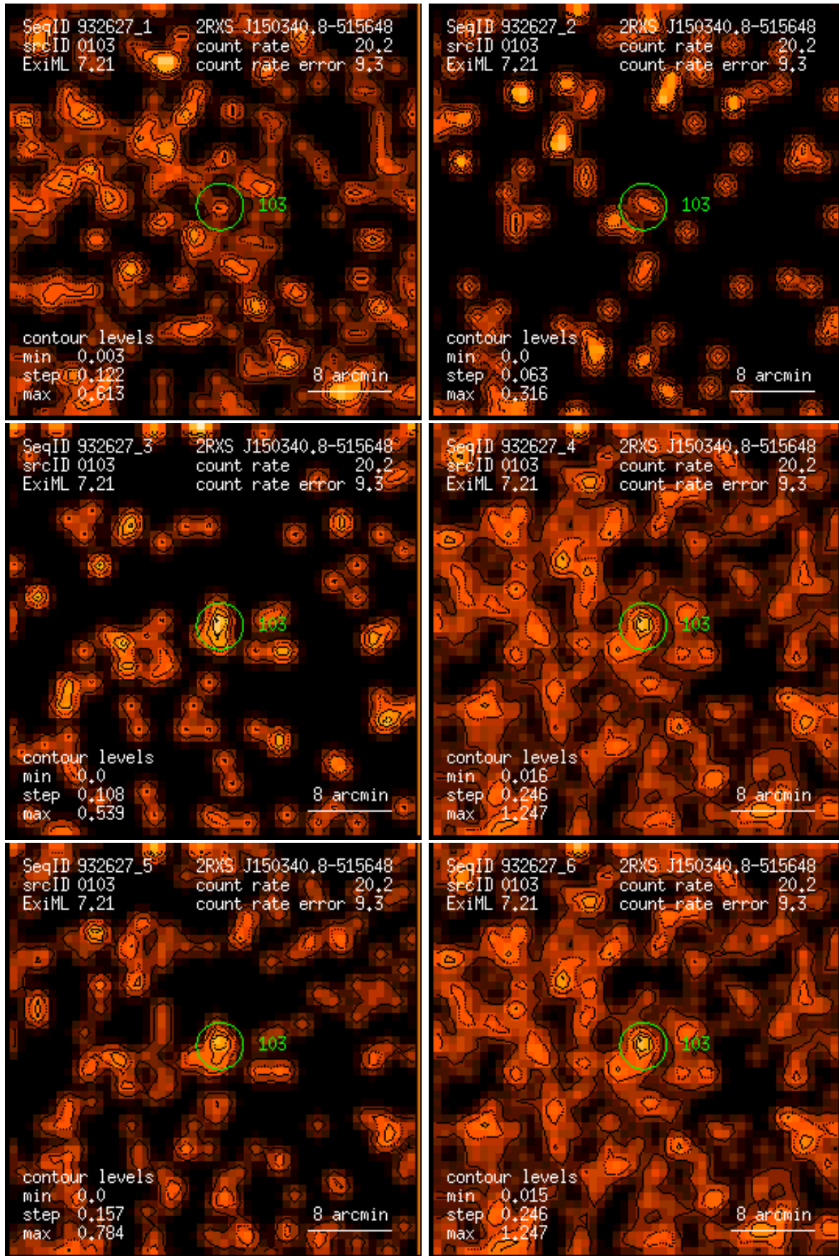
Figure 103: RASS 932627: detection 0103: band rate images, Gaussian filter: (1) PSPC channels 11 – 41, (2) 52 – 90, (3) 91 – 201, (4) 11 – 235, (5) 52 – 201, (6) 11 – 201. Broad band rates in counts/ks. Band rate contour levels in counts/ks/arcmin 2 .
