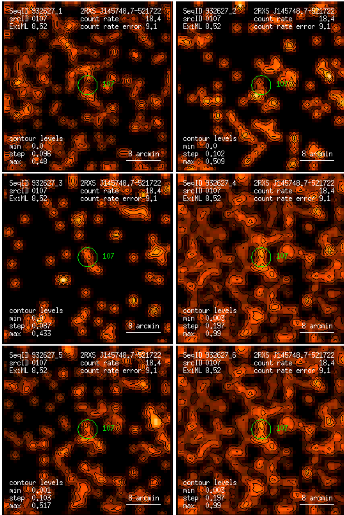
Figure 107: RASS 932627: detection 0107: band rate images, Gaussian filter: (1) PSPC channels 11 – 41, (2) 52 – 90, (3) 91 – 201, (4) 11 – 235, (5) 52 – 201, (6) 11 – 201. Broad band rates in counts/ks. Band rate contour levels in counts/ks/arcmin 2 .
