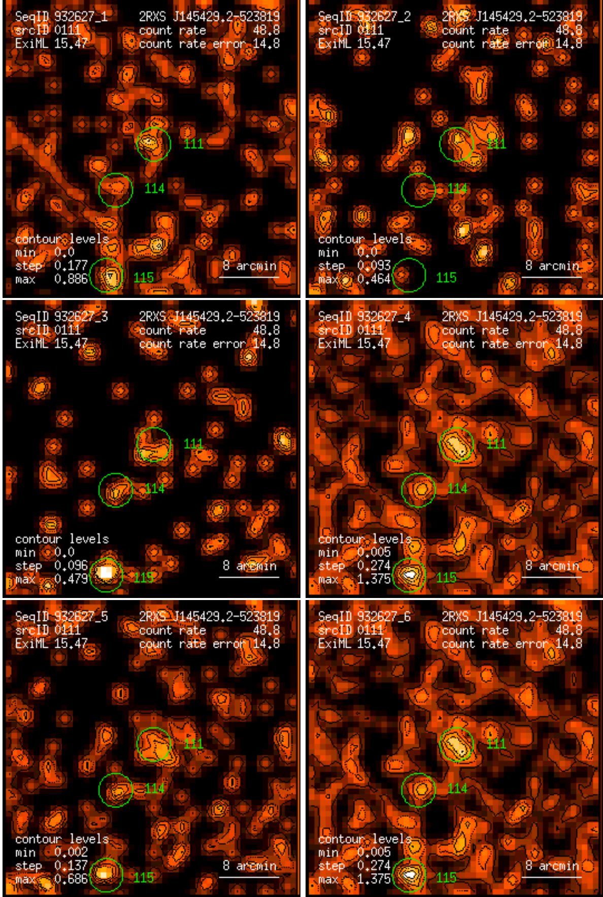
Figure 111: RASS 932627: detection 0111: band rate images, Gaussian filter: (1) PSPC channels 11 – 41, (2) 52 – 90, (3) 91 – 201, (4) 11 – 235, (5) 52 – 201, (6) 11 – 201. Broad band rates in counts/ks. Band rate contour levels in counts/ks/arcmin 2 .
