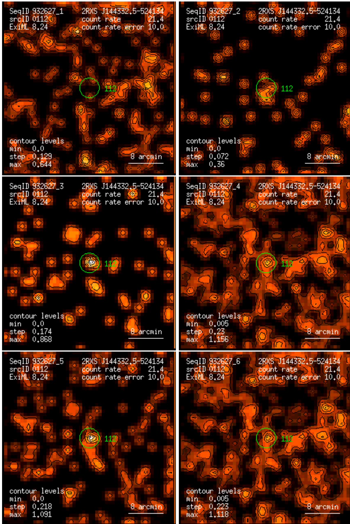
Figure 112: RASS 932627: detection 0112: band rate images, Gaussian filter: (1) PSPC channels 11 – 41, (2) 52 – 90, (3) 91 – 201, (4) 11 – 235, (5) 52 – 201, (6) 11 – 201. Broad band rates in counts/ks. Band rate contour levels in counts/ks/arcmin 2 .
