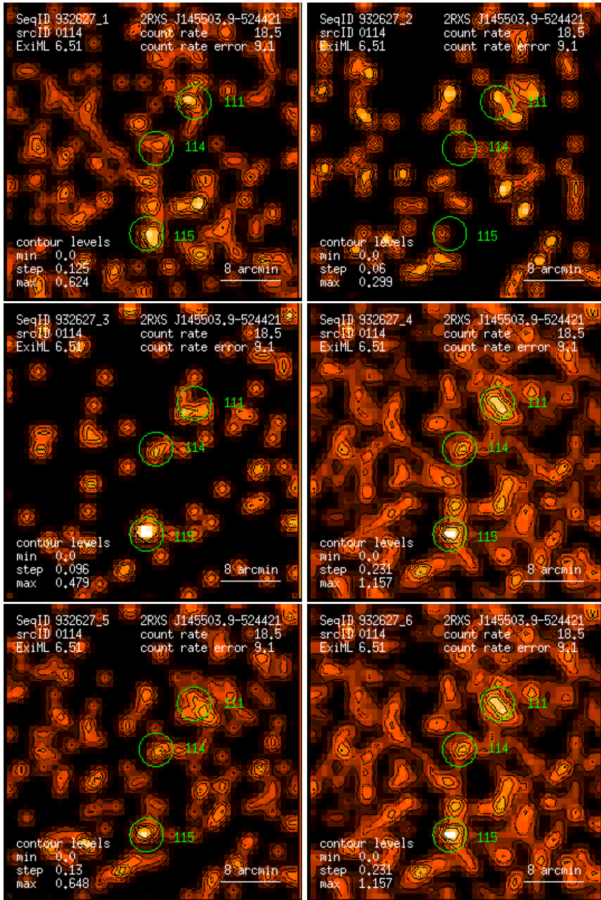
Figure 114: RASS 932627: detection 0114: band rate images, Gaussian filter: (1) PSPC channels 11 – 41, (2) 52 – 90, (3) 91 – 201, (4) 11 – 235, (5) 52 – 201, (6) 11 – 201. Broad band rates in counts/ks. Band rate contour levels in counts/ks/arcmin 2 .
