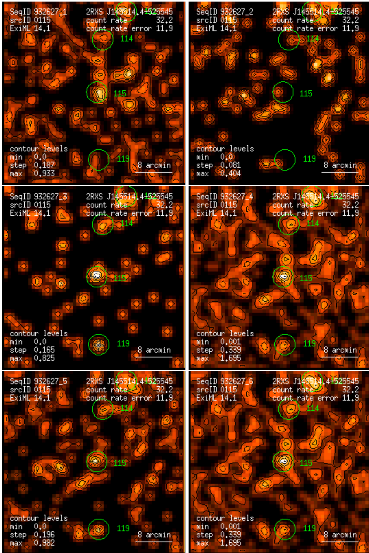
Figure 115: RASS 932627: detection 0115: band rate images, Gaussian filter: (1) PSPC channels 11 – 41, (2) 52 – 90, (3) 91 – 201, (4) 11 – 235, (5) 52 – 201, (6) 11 – 201. Broad band rates in counts/ks. Band rate contour levels in counts/ks/arcmin 2 .
