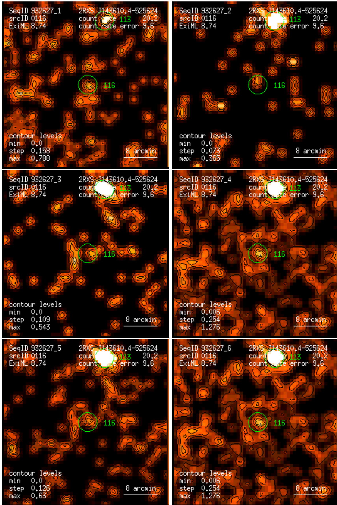
Figure 116: RASS 932627: detection 0116: band rate images, Gaussian filter: (1) PSPC channels 11 – 41, (2) 52 – 90, (3) 91 – 201, (4) 11 – 235, (5) 52 – 201, (6) 11 – 201. Broad band rates in counts/ks. Band rate contour levels in counts/ks/arcmin 2 .
