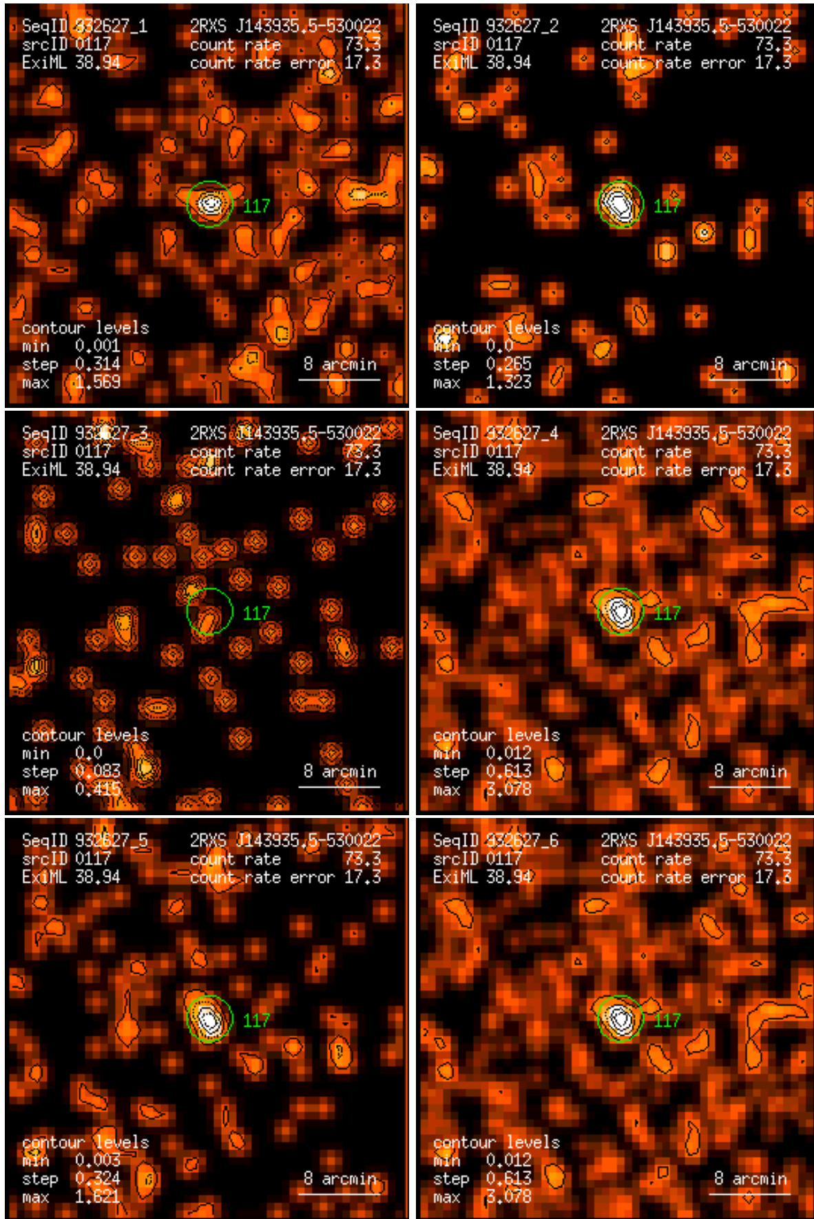
Figure 117: RASS 932627: detection 0117: band rate images, Gaussian filter: (1) PSPC channels 11 – 41, (2) 52 – 90, (3) 91 – 201, (4) 11 – 235, (5) 52 – 201, (6) 11 – 201. Broad band rates in counts/ks. Band rate contour levels in counts/ks/arcmin 2 .
