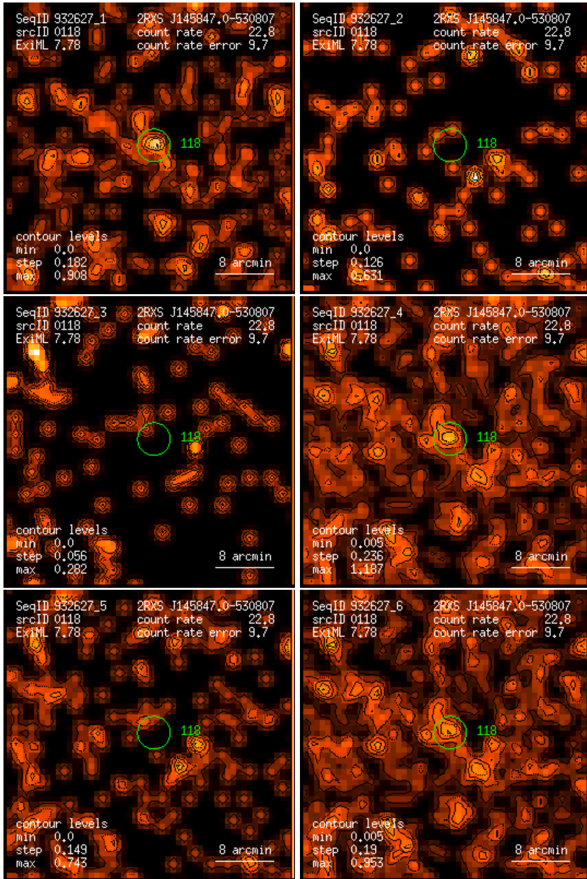
Figure 118: RASS 932627: detection 0118: band rate images, Gaussian filter: (1) PSPC channels 11 – 41, (2) 52 – 90, (3) 91 – 201, (4) 11 – 235, (5) 52 – 201, (6) 11 – 201. Broad band rates in counts/ks. Band rate contour levels in counts/ks/arcmin 2 .
