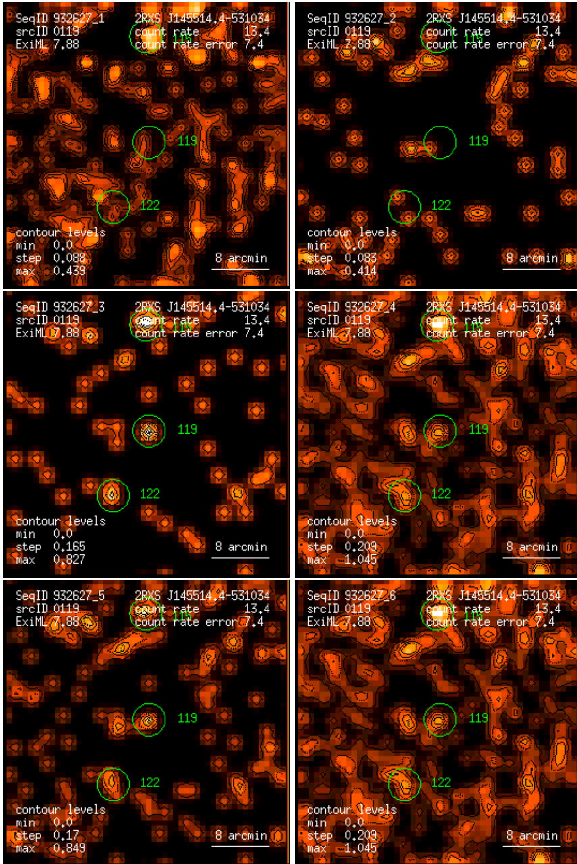
Figure 119: RASS 932627: detection 0119: band rate images, Gaussian filter: (1) PSPC channels 11 – 41, (2) 52 – 90, (3) 91 – 201, (4) 11 – 235, (5) 52 – 201, (6) 11 – 201. Broad band rates in counts/ks. Band rate contour levels in counts/ks/arcmin 2 .
