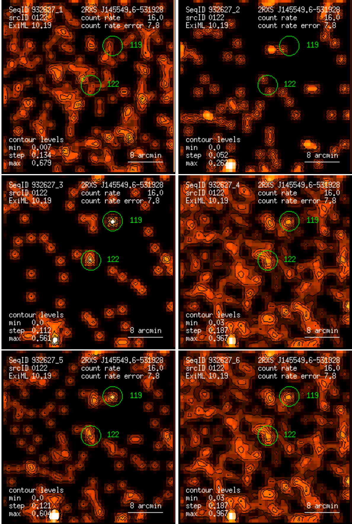
Figure 122: RASS 932627: detection 0122: band rate images, Gaussian filter: (1) PSPC channels 11 – 41, (2) 52 – 90, (3) 91 – 201, (4) 11 – 235, (5) 52 – 201, (6) 11 – 201. Broad band rates in counts/ks. Band rate contour levels in counts/ks/arcmin 2 .
