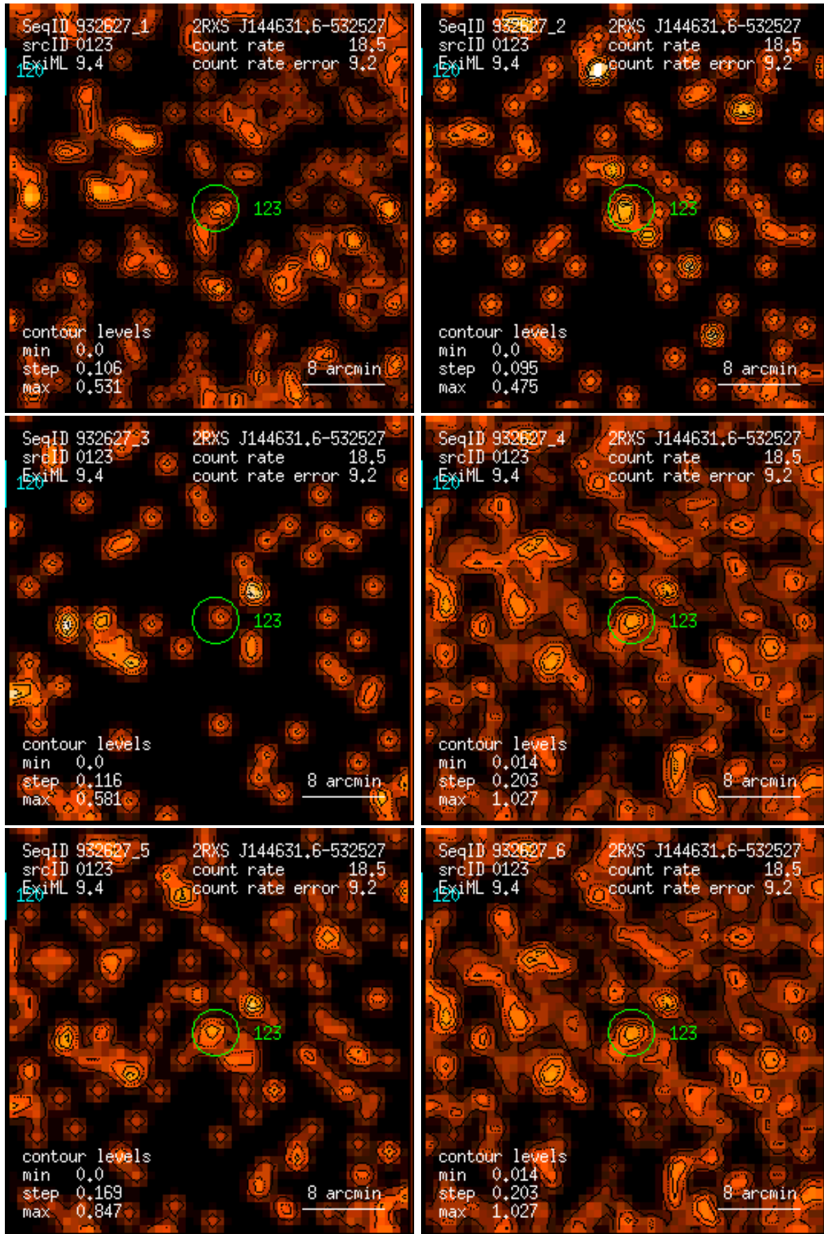
Figure 123: RASS 932627: detection 0123: band rate images, Gaussian filter: (1) PSPC channels 11 – 41, (2) 52 – 90, (3) 91 – 201, (4) 11 – 235, (5) 52 – 201, (6) 11 – 201. Broad band rates in counts/ks. Band rate contour levels in counts/ks/arcmin 2 .
