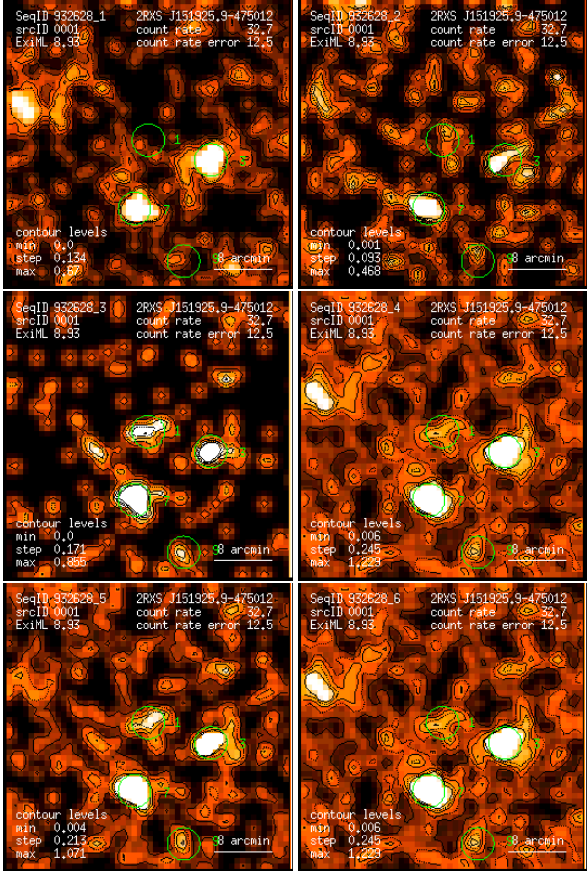
Figure 1: RASS 932628: detection 0001: band rate images, Gaussian filter: (1) PSPC channels 11 – 41, (2) 52 – 90, (3) 91 – 201, (4) 11 – 235, (5) 52 – 201, (6) 11 – 201. Broad band rates in counts/ks. Band rate contour levels in counts/ks/arcmin 2 .
