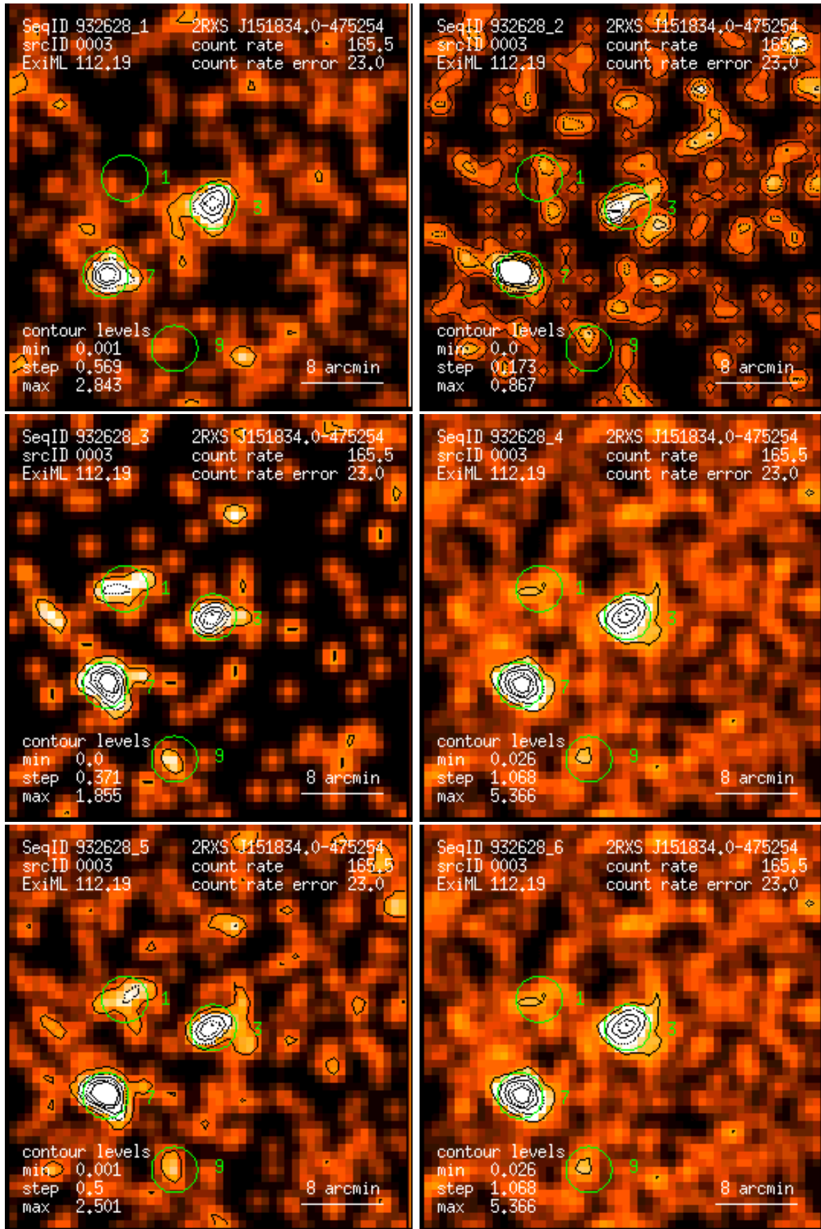
Figure 3: RASS 932628: detection 0003: band rate images, Gaussian filter: (1) PSPC channels 11 – 41, (2) 52 – 90, (3) 91 – 201, (4) 11 – 235, (5) 52 – 201, (6) 11 – 201. Broad band rates in counts/ks. Band rate contour levels in counts/ks/arcmin 2 .
