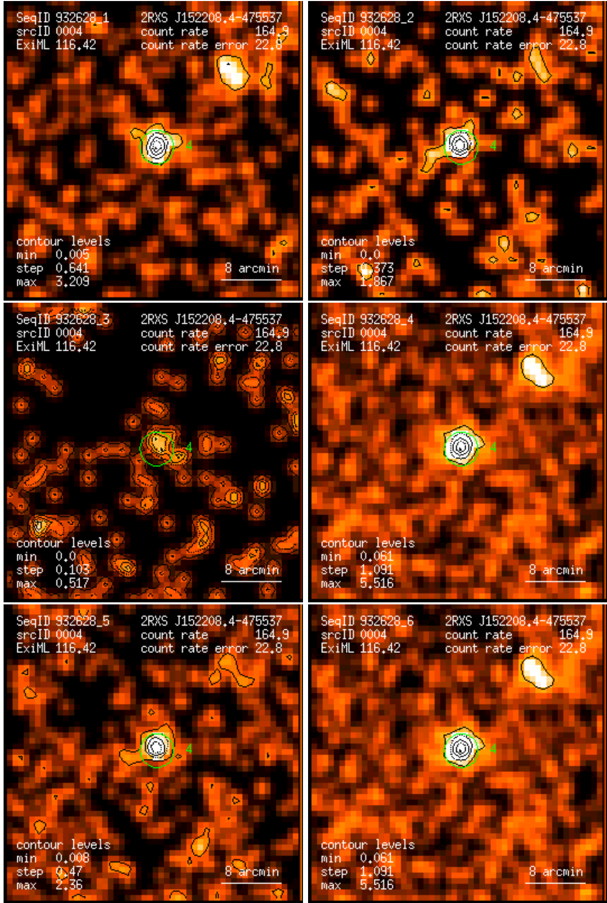
Figure 4: RASS 932628: detection 0004: band rate images, Gaussian filter: (1) PSPC channels 11 – 41, (2) 52 – 90, (3) 91 – 201, (4) 11 – 235, (5) 52 – 201, (6) 11 – 201. Broad band rates in counts/ks. Band rate contour levels in counts/ks/arcmin 2 .
