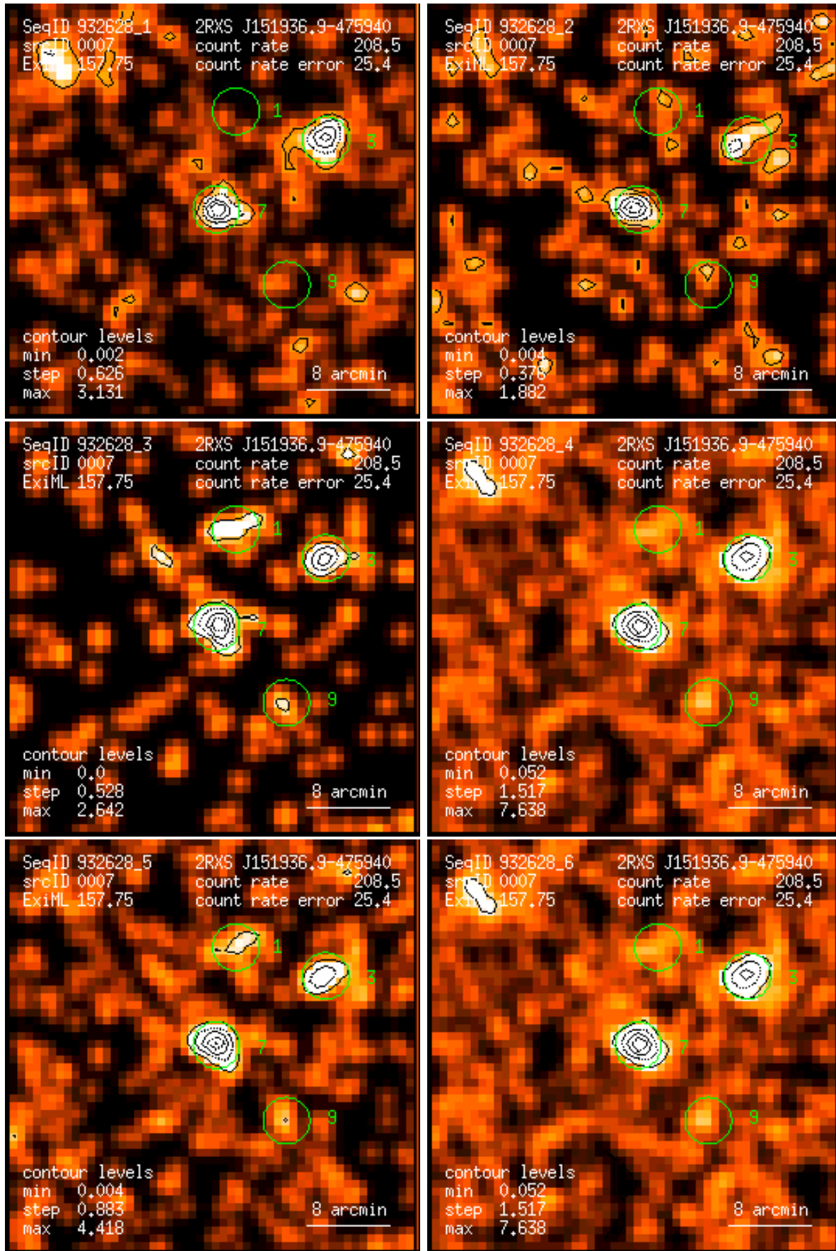
Figure 7: RASS 932628: detection 0007: band rate images, Gaussian filter: (1) PSPC channels 11 – 41, (2) 52 – 90, (3) 91 – 201, (4) 11 – 235, (5) 52 – 201, (6) 11 – 201. Broad band rates in counts/ks. Band rate contour levels in counts/ks/arcmin 2 .
