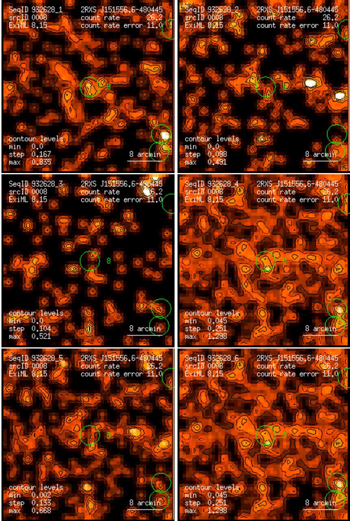
Figure 8: RASS 932628: detection 0008: band rate images, Gaussian filter: (1) PSPC channels 11 – 41, (2) 52 – 90, (3) 91 – 201, (4) 11 – 235, (5) 52 – 201, (6) 11 – 201. Broad band rates in counts/ks. Band rate contour levels in counts/ks/arcmin 2 .
