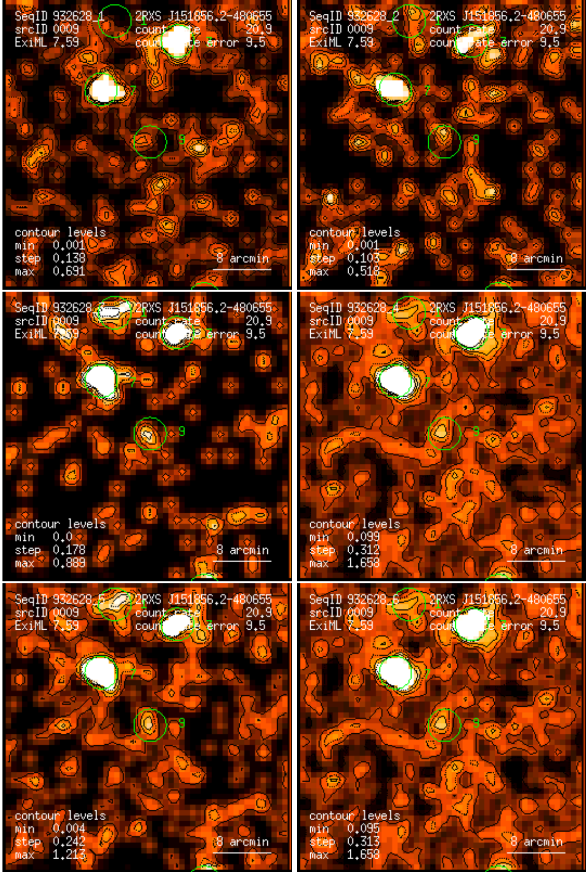
Figure 9: RASS 932628: detection 0009: band rate images, Gaussian filter: (1) PSPC channels 11 – 41, (2) 52 – 90, (3) 91 – 201, (4) 11 – 235, (5) 52 – 201, (6) 11 – 201. Broad band rates in counts/ks. Band rate contour levels in counts/ks/arcmin 2 .
