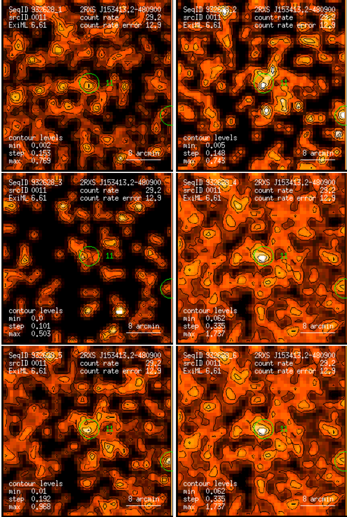
Figure 11: RASS 932628: detection 0011: band rate images, Gaussian filter: (1) PSPC channels 11 – 41, (2) 52 – 90, (3) 91 – 201, (4) 11 – 235, (5) 52 – 201, (6) 11 – 201. Broad band rates in counts/ks. Band rate contour levels in counts/ks/arcmin 2 .
