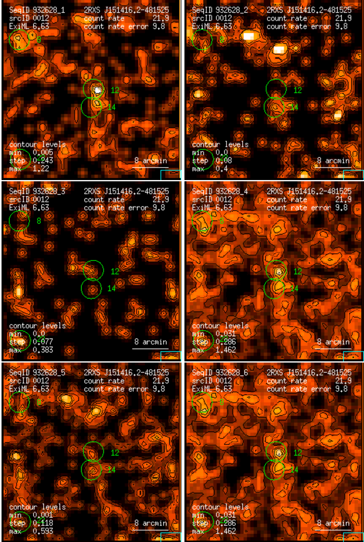
Figure 12: RASS 932628: detection 0012: band rate images, Gaussian filter: (1) PSPC channels 11 – 41, (2) 52 – 90, (3) 91 – 201, (4) 11 – 235, (5) 52 – 201, (6) 11 – 201. Broad band rates in counts/ks. Band rate contour levels in counts/ks/arcmin 2 .
