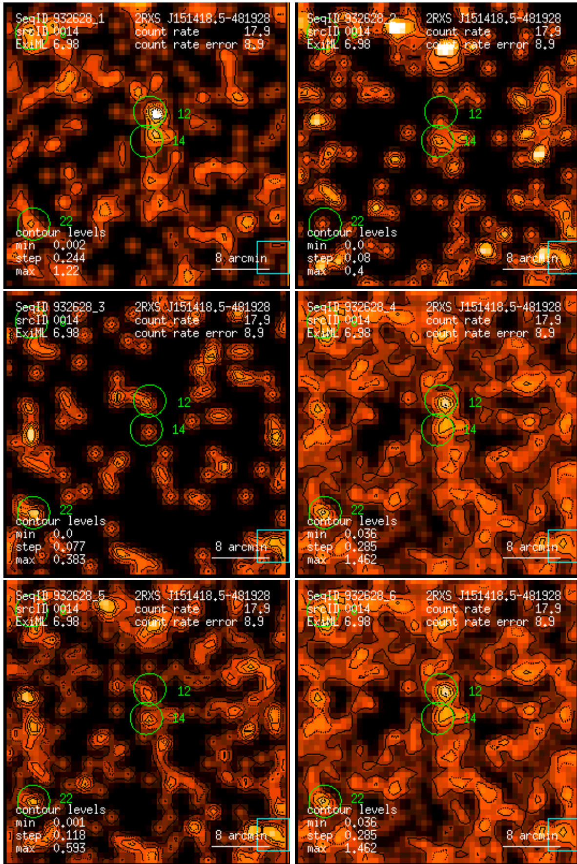
Figure 14: RASS 932628: detection 0014: band rate images, Gaussian filter: (1) PSPC channels 11 – 41, (2) 52 – 90, (3) 91 – 201, (4) 11 – 235, (5) 52 – 201, (6) 11 – 201. Broad band rates in counts/ks. Band rate contour levels in counts/ks/arcmin 2 .
