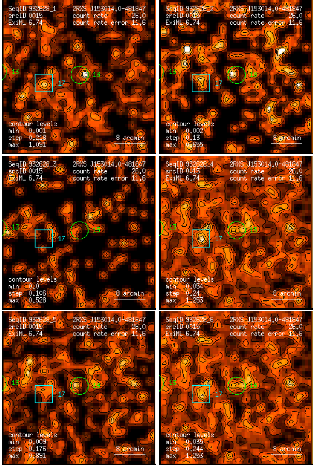
Figure 15: RASS 932628: detection 0015: band rate images, Gaussian filter: (1) PSPC channels 11 – 41, (2) 52 – 90, (3) 91 – 201, (4) 11 – 235, (5) 52 – 201, (6) 11 – 201. Broad band rates in counts/ks. Band rate contour levels in counts/ks/arcmin 2 .
