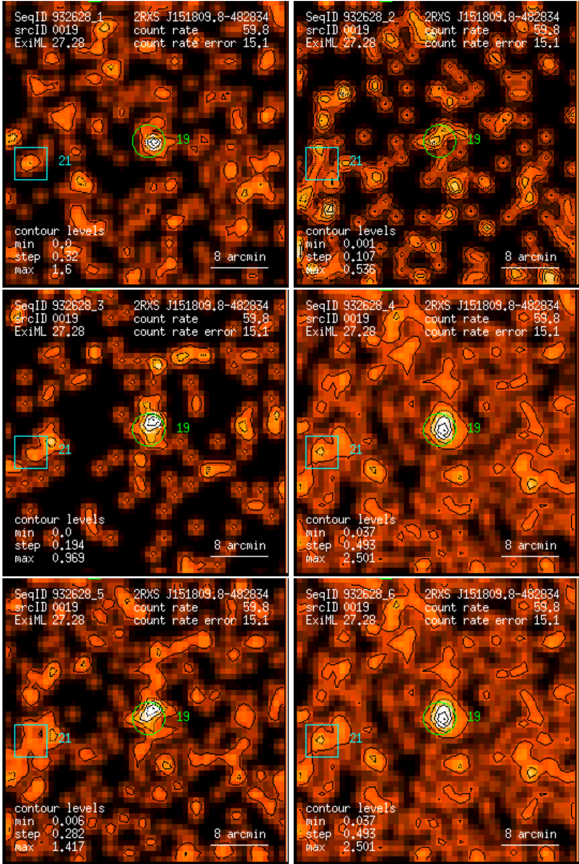
Figure 19: RASS 932628: detection 0019: band rate images, Gaussian filter: (1) PSPC channels 11 – 41, (2) 52 – 90, (3) 91 – 201, (4) 11 – 235, (5) 52 – 201, (6) 11 – 201. Broad band rates in counts/ks. Band rate contour levels in counts/ks/arcmin 2 .
