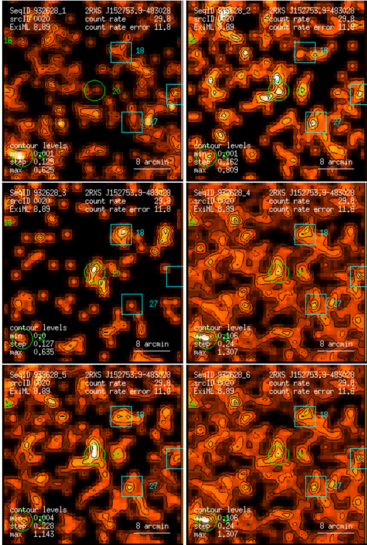
Figure 20: RASS 932628: detection 0020: band rate images, Gaussian filter: (1) PSPC channels 11 – 41, (2) 52 – 90, (3) 91 – 201, (4) 11 – 235, (5) 52 – 201, (6) 11 – 201. Broad band rates in counts/ks. Band rate contour levels in counts/ks/arcmin 2 .
