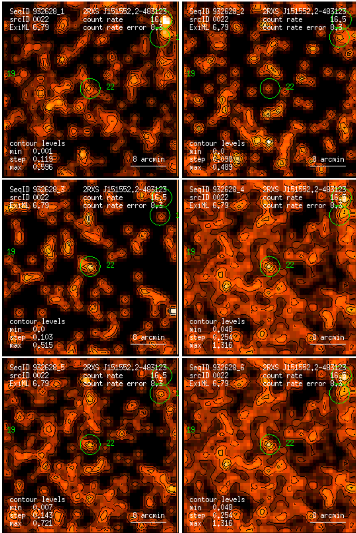
Figure 22: RASS 932628: detection 0022: band rate images, Gaussian filter: (1) PSPC channels 11 – 41, (2) 52 – 90, (3) 91 – 201, (4) 11 – 235, (5) 52 – 201, (6) 11 – 201. Broad band rates in counts/ks. Band rate contour levels in counts/ks/arcmin 2 .
