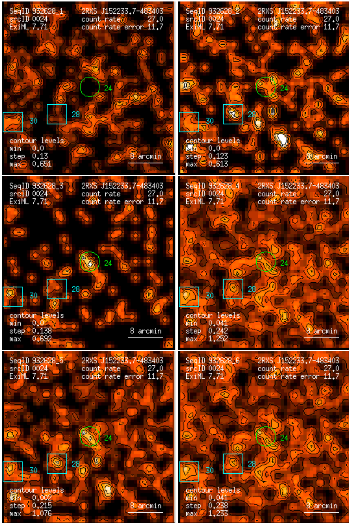
Figure 24: RASS 932628: detection 0024: band rate images, Gaussian filter: (1) PSPC channels 11 – 41, (2) 52 – 90, (3) 91 – 201, (4) 11 – 235, (5) 52 – 201, (6) 11 – 201. Broad band rates in counts/ks. Band rate contour levels in counts/ks/arcmin 2 .
