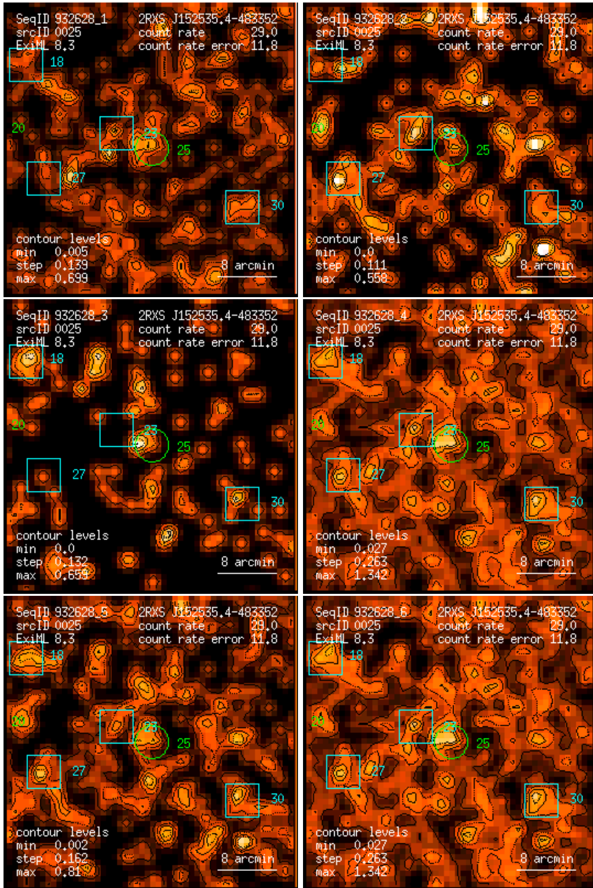
Figure 25: RASS 932628: detection 0025: band rate images, Gaussian filter: (1) PSPC channels 11 – 41, (2) 52 – 90, (3) 91 – 201, (4) 11 – 235, (5) 52 – 201, (6) 11 – 201. Broad band rates in counts/ks. Band rate contour levels in counts/ks/arcmin 2 .
