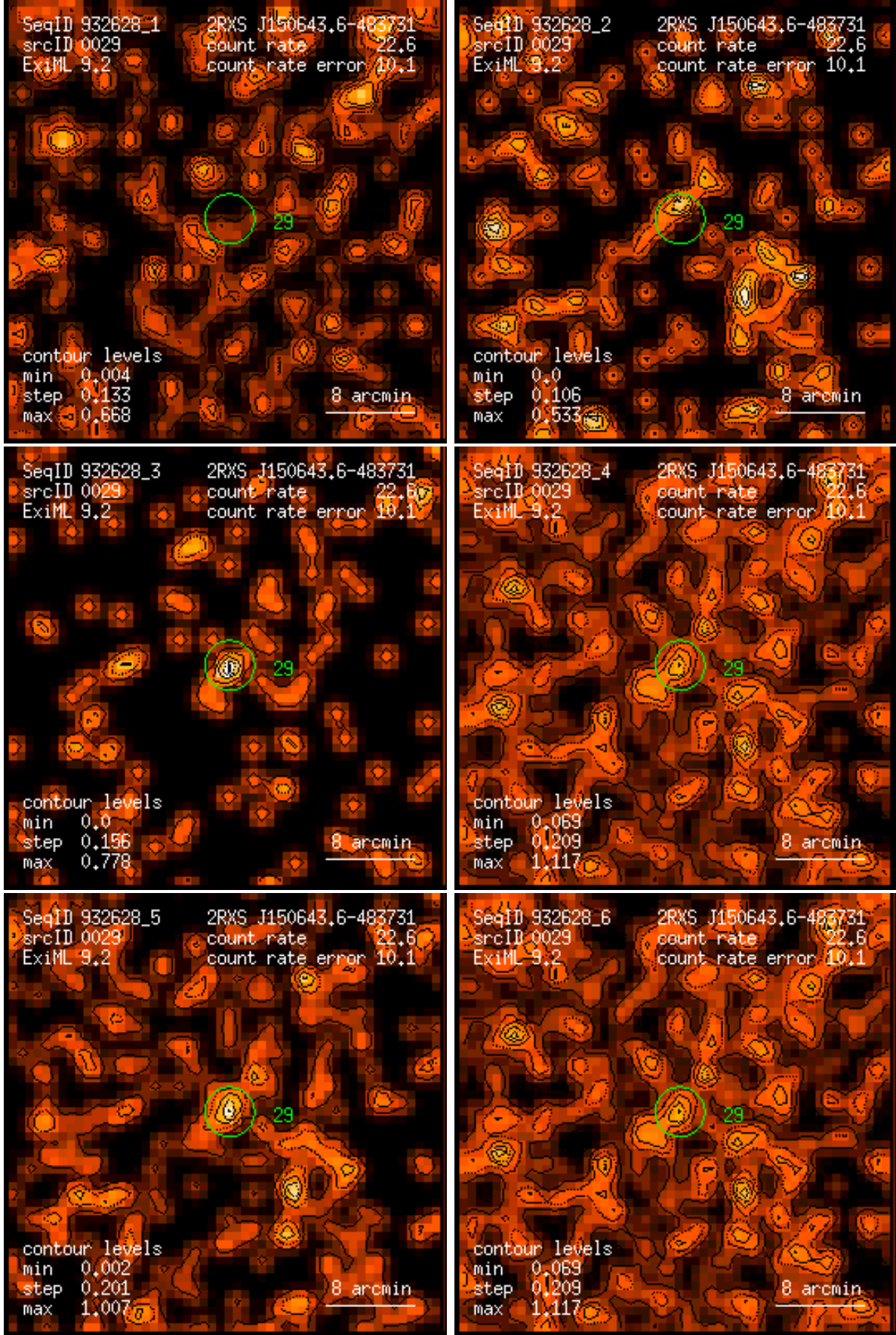
Figure 29: RASS 932628: detection 0029: band rate images, Gaussian filter: (1) PSPC channels 11 – 41, (2) 52 – 90, (3) 91 – 201, (4) 11 – 235, (5) 52 – 201, (6) 11 – 201. Broad band rates in counts/ks. Band rate contour levels in counts/ks/arcmin 2 .
