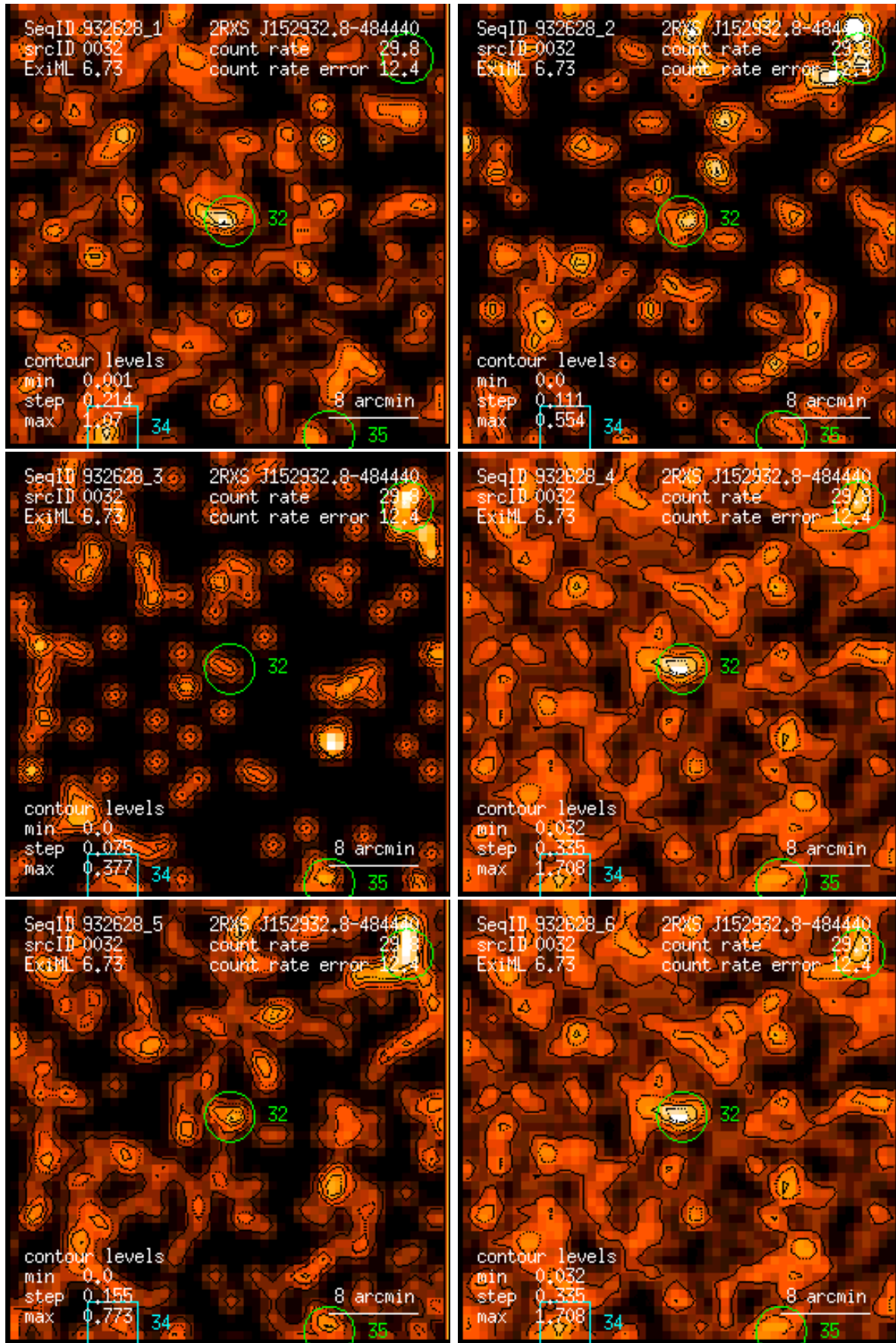
Figure 32: RASS 932628: detection 0032: band rate images, Gaussian filter: (1) PSPC channels 11 – 41, (2) 52 – 90, (3) 91 – 201, (4) 11 – 235, (5) 52 – 201, (6) 11 – 201. Broad band rates in counts/ks. Band rate contour levels in counts/ks/arcmin 2 .
