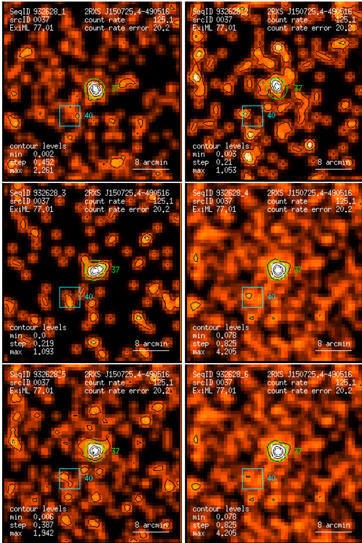
Figure 37: RASS 932628: detection 0037: band rate images, Gaussian filter: (1) PSPC channels 11 – 41, (2) 52 – 90, (3) 91 – 201, (4) 11 – 235, (5) 52 – 201, (6) 11 – 201. Broad band rates in counts/ks. Band rate contour levels in counts/ks/arcmin 2 .
