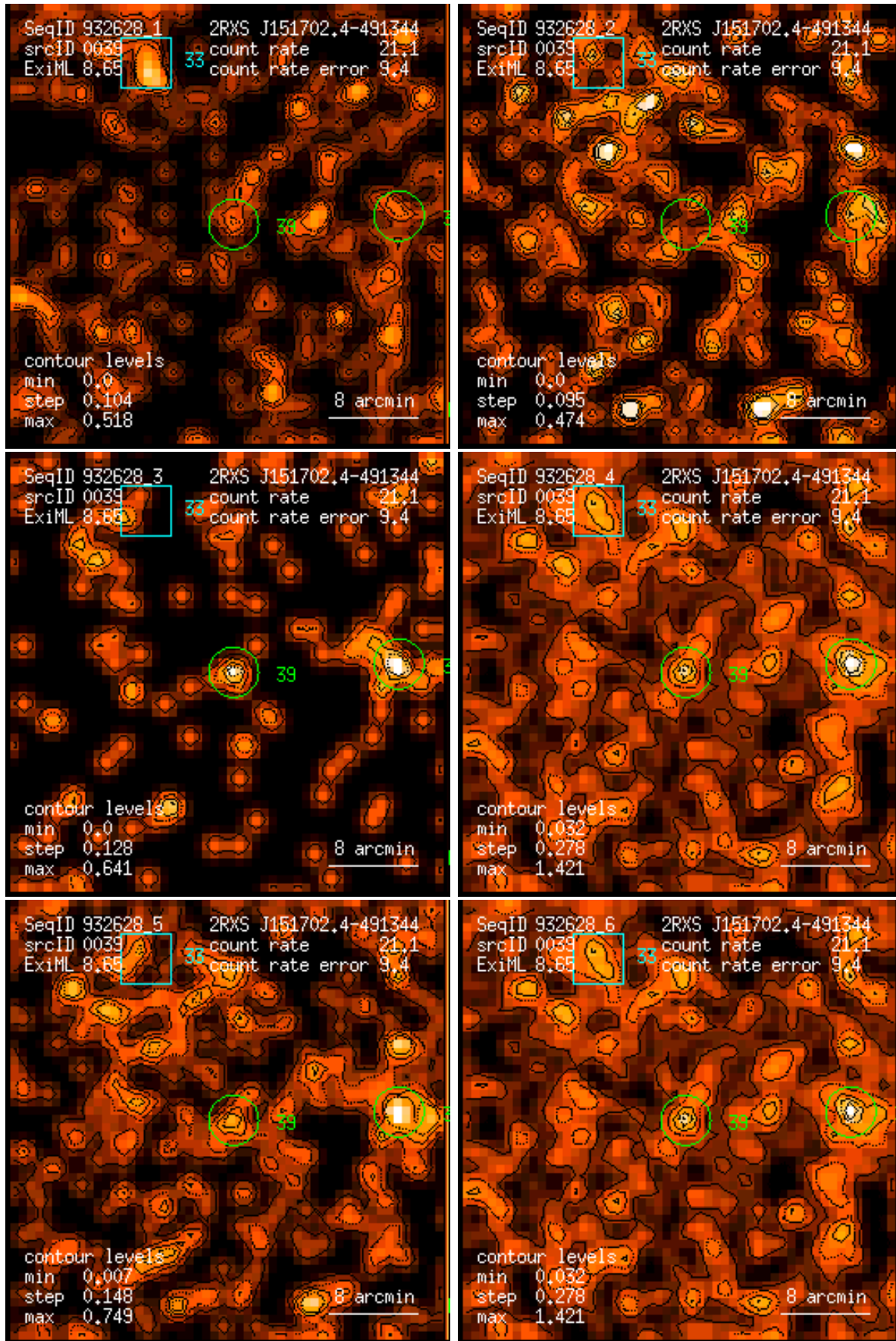
Figure 39: RASS 932628: detection 0039: band rate images, Gaussian filter: (1) PSPC channels 11 – 41, (2) 52 – 90, (3) 91 – 201, (4) 11 – 235, (5) 52 – 201, (6) 11 – 201. Broad band rates in counts/ks. Band rate contour levels in counts/ks/arcmin 2 .
