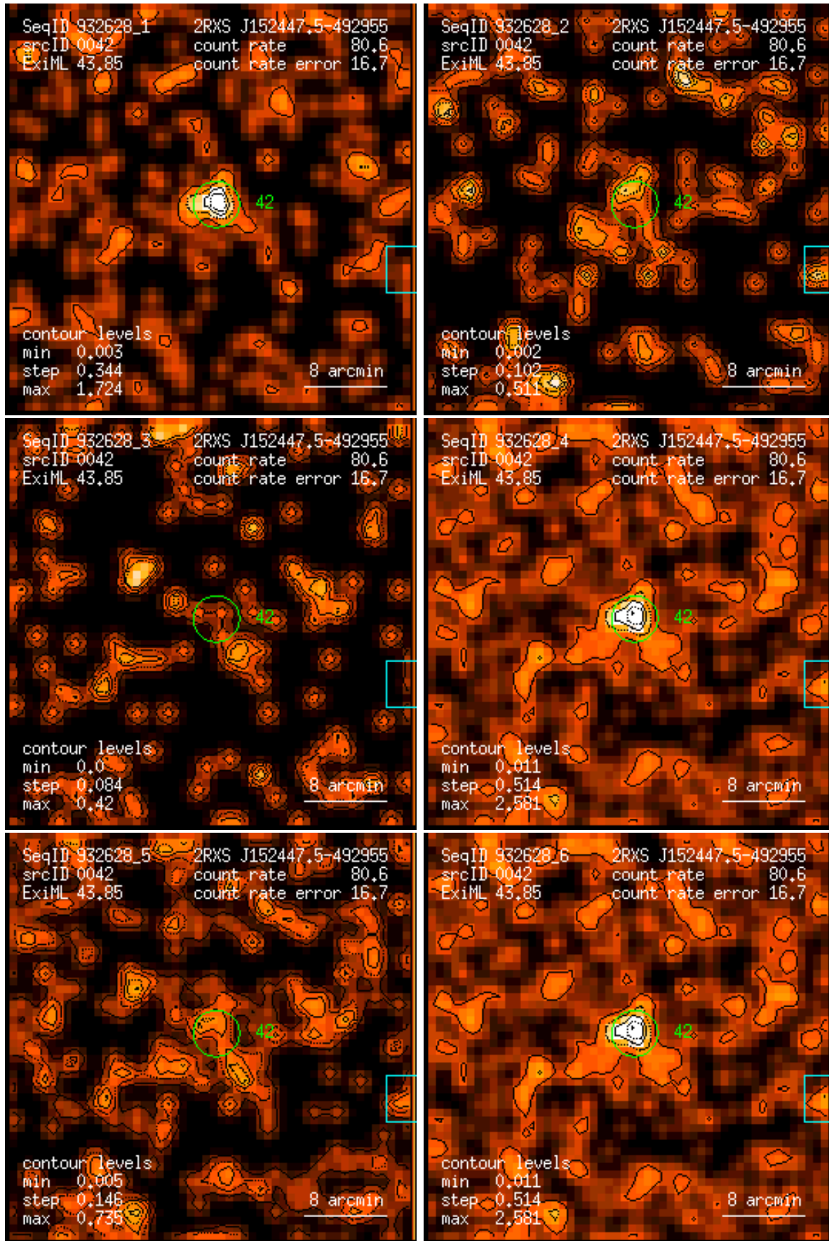
Figure 42: RASS 932628: detection 0042: band rate images, Gaussian filter: (1) PSPC channels 11 – 41, (2) 52 – 90, (3) 91 – 201, (4) 11 – 235, (5) 52 – 201, (6) 11 – 201. Broad band rates in counts/ks. Band rate contour levels in counts/ks/arcmin 2 .
