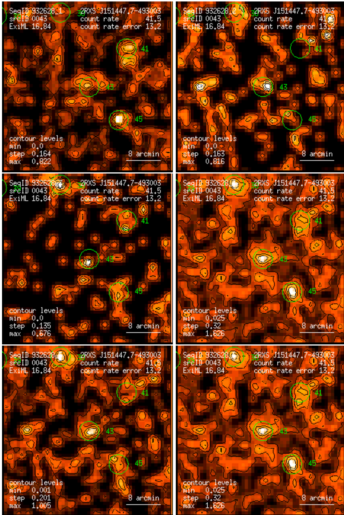
Figure 43: RASS 932628: detection 0043: band rate images, Gaussian filter: (1) PSPC channels 11 – 41, (2) 52 – 90, (3) 91 – 201, (4) 11 – 235, (5) 52 – 201, (6) 11 – 201. Broad band rates in counts/ks. Band rate contour levels in counts/ks/arcmin 2 .
