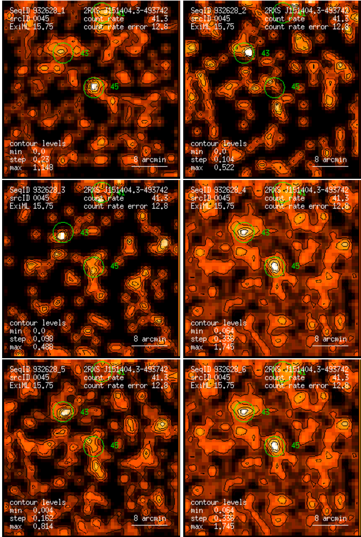
Figure 45: RASS 932628: detection 0045: band rate images, Gaussian filter: (1) PSPC channels 11 – 41, (2) 52 – 90, (3) 91 – 201, (4) 11 – 235, (5) 52 – 201, (6) 11 – 201. Broad band rates in counts/ks. Band rate contour levels in counts/ks/arcmin 2 .
