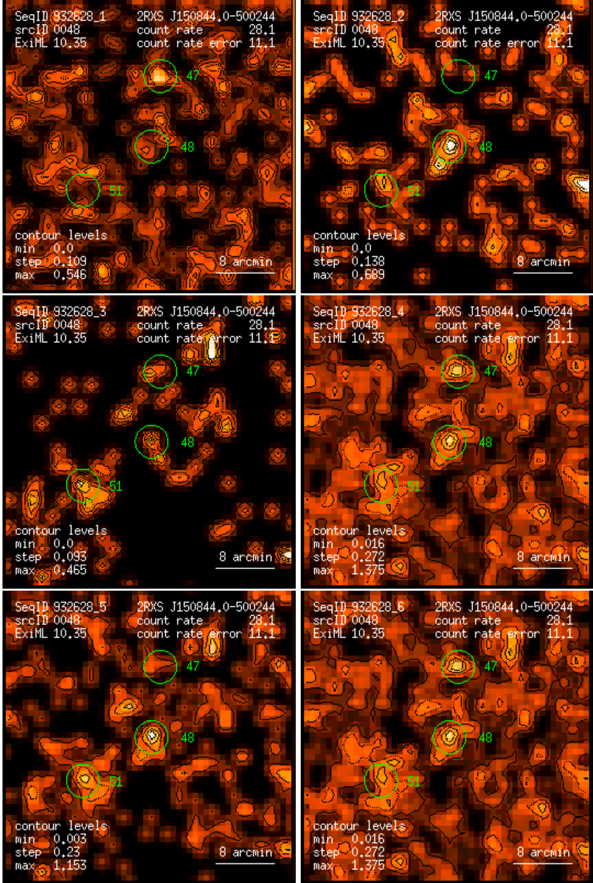
Figure 48: RASS 932628: detection 0048: band rate images, Gaussian filter: (1) PSPC channels 11 – 41, (2) 52 – 90, (3) 91 – 201, (4) 11 – 235, (5) 52 – 201, (6) 11 – 201. Broad band rates in counts/ks. Band rate contour levels in counts/ks/arcmin 2 .
