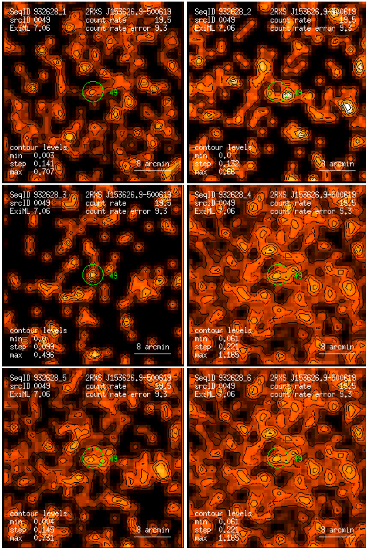
Figure 49: RASS 932628: detection 0049: band rate images, Gaussian filter: (1) PSPC channels 11 – 41, (2) 52 – 90, (3) 91 – 201, (4) 11 – 235, (5) 52 – 201, (6) 11 – 201. Broad band rates in counts/ks. Band rate contour levels in counts/ks/arcmin 2 .
