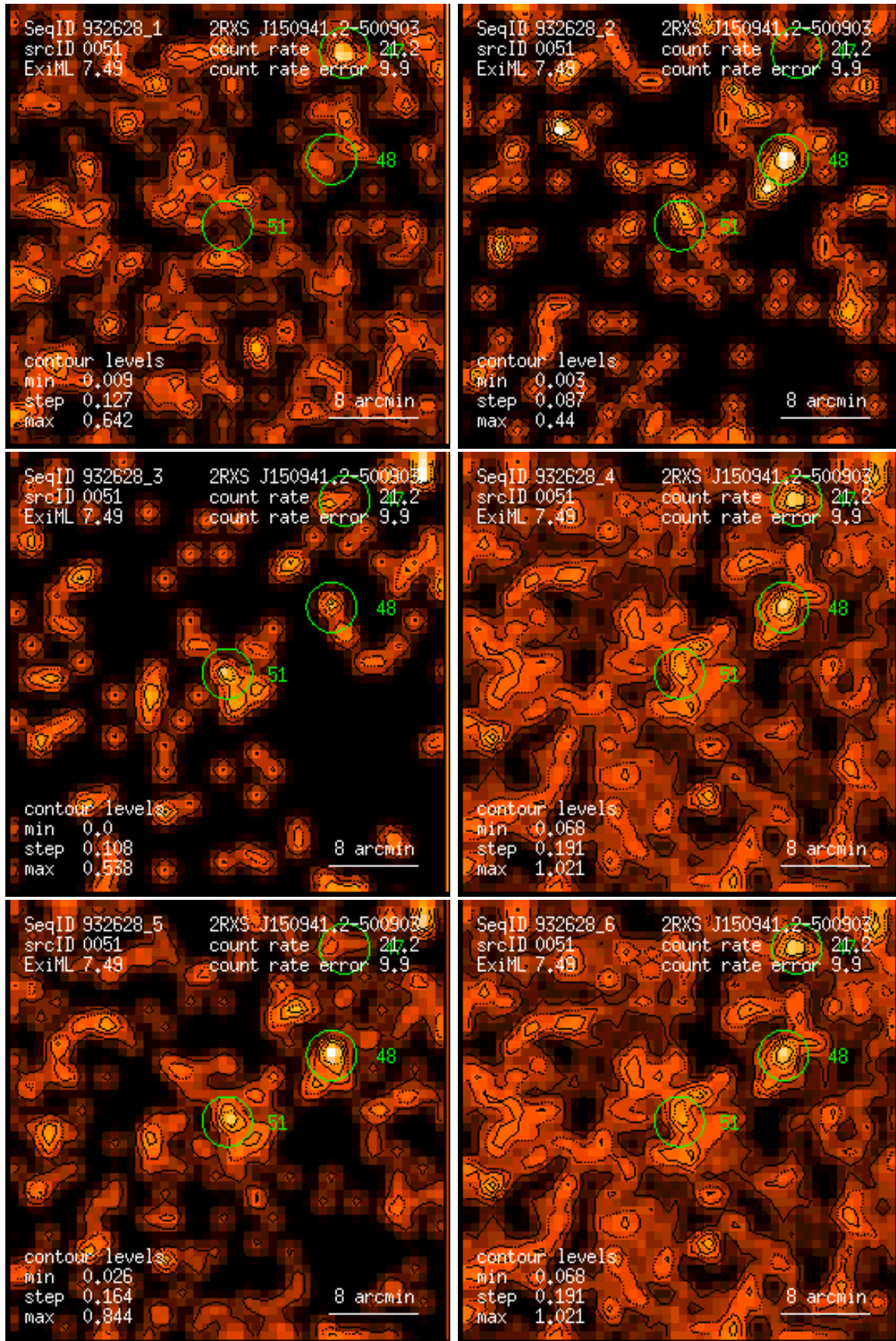
Figure 51: RASS 932628: detection 0051: band rate images, Gaussian filter: (1) PSPC channels 11 – 41, (2) 52 – 90, (3) 91 – 201, (4) 11 – 235, (5) 52 – 201, (6) 11 – 201. Broad band rates in counts/ks. Band rate contour levels in counts/ks/arcmin 2 .
