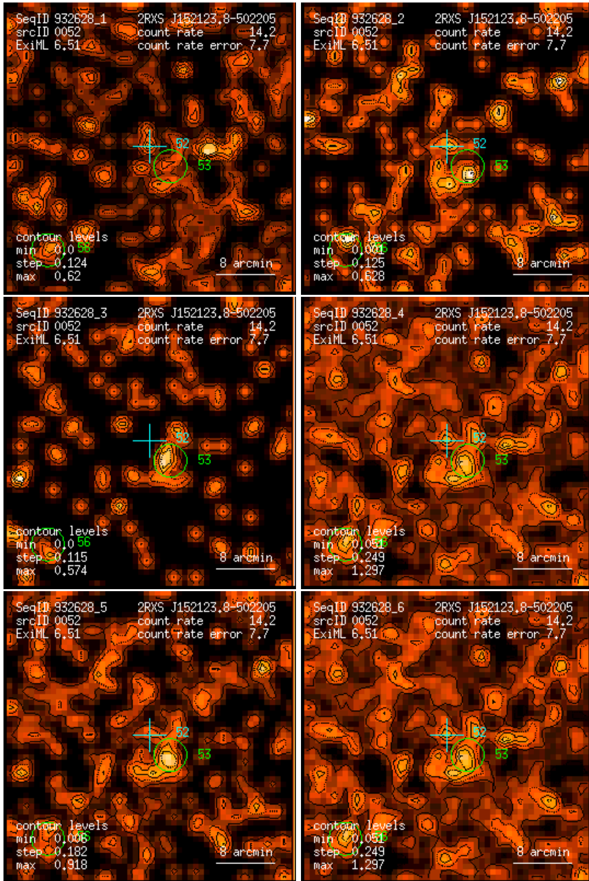
Figure 52: RASS 932628: detection 0052: band rate images, Gaussian filter: (1) PSPC channels 11 – 41, (2) 52 – 90, (3) 91 – 201, (4) 11 – 235, (5) 52 – 201, (6) 11 – 201. Broad band rates in counts/ks. Band rate contour levels in counts/ks/arcmin 2 .
