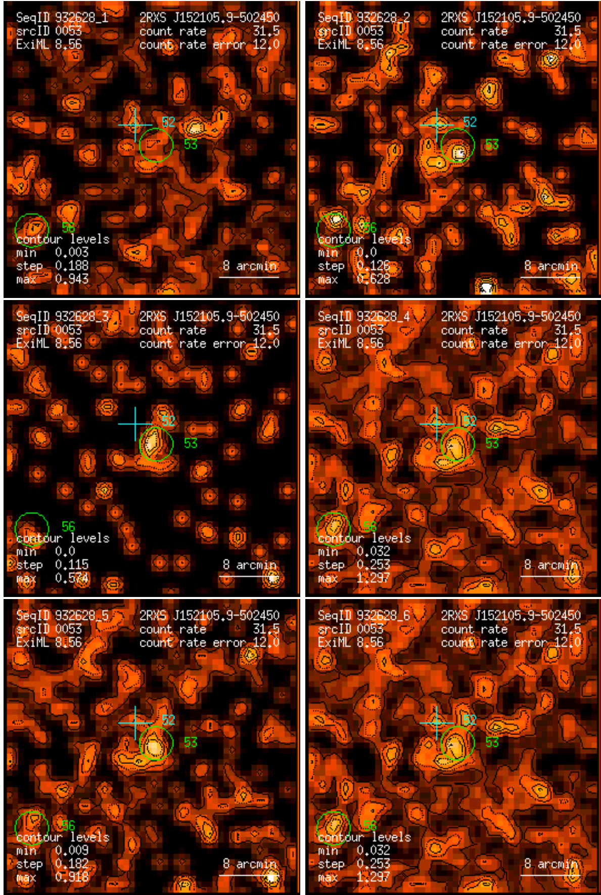
Figure 53: RASS 932628: detection 0053: band rate images, Gaussian filter: (1) PSPC channels 11 – 41, (2) 52 – 90, (3) 91 – 201, (4) 11 – 235, (5) 52 – 201, (6) 11 – 201. Broad band rates in counts/ks. Band rate contour levels in counts/ks/arcmin 2 .
