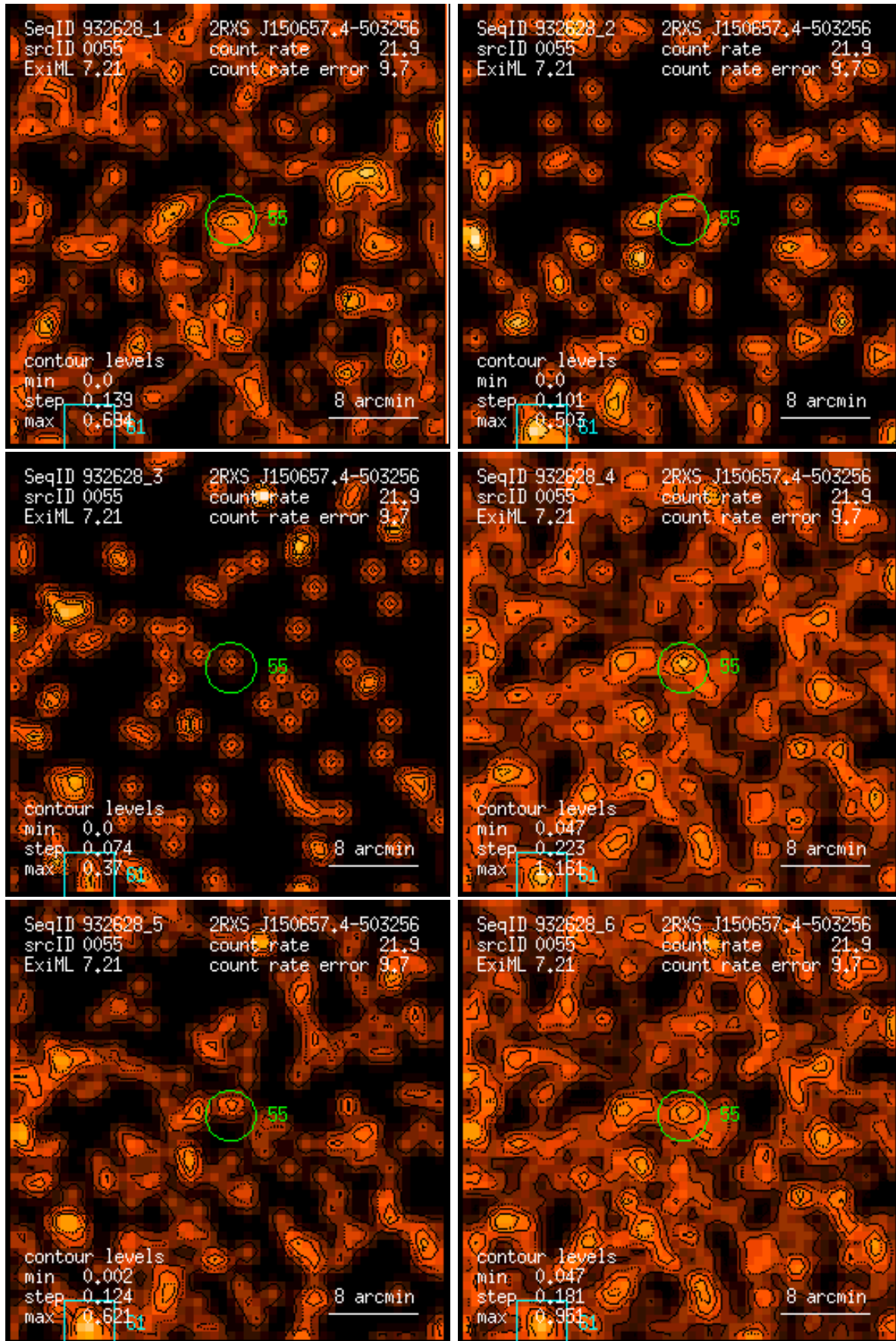
Figure 55: RASS 932628: detection 0055: band rate images, Gaussian filter: (1) PSPC channels 11 – 41, (2) 52 – 90, (3) 91 – 201, (4) 11 – 235, (5) 52 – 201, (6) 11 – 201. Broad band rates in counts/ks. Band rate contour levels in counts/ks/arcmin 2 .
