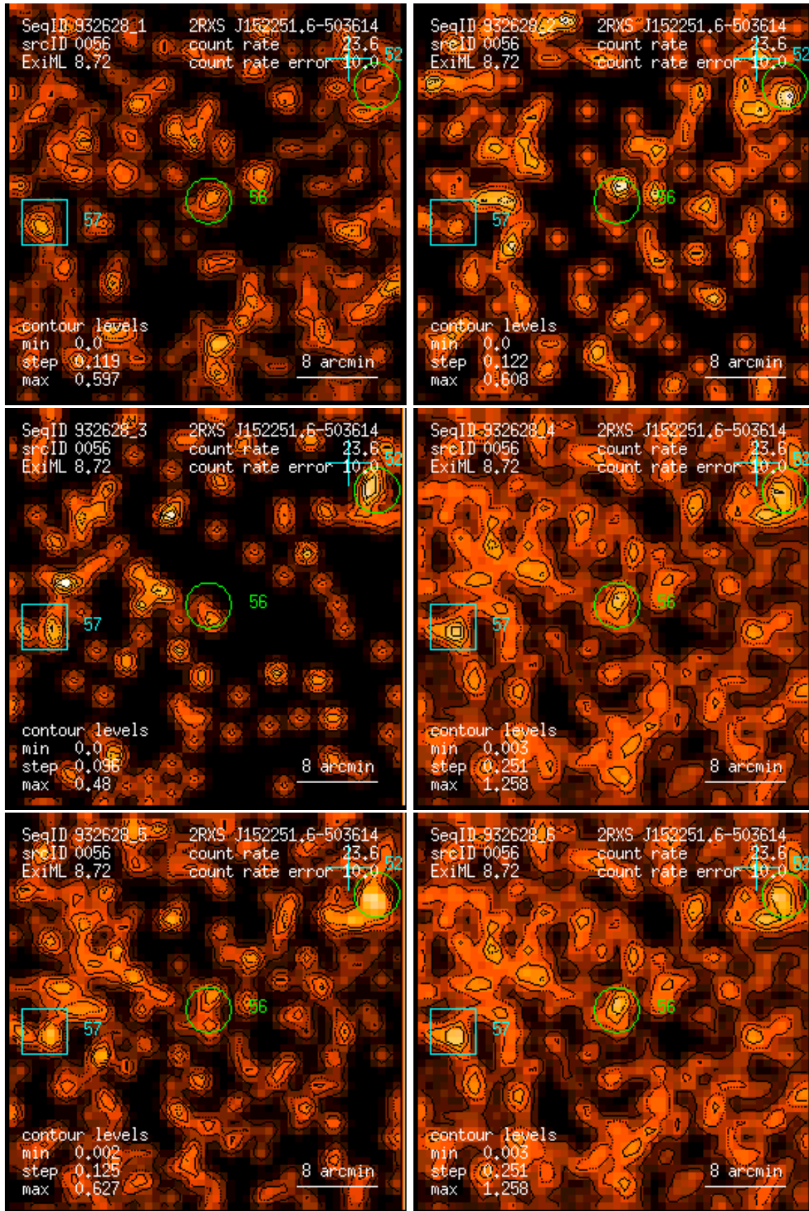
Figure 56: RASS 932628: detection 0056: band rate images, Gaussian filter: (1) PSPC channels 11 – 41, (2) 52 – 90, (3) 91 – 201, (4) 11 – 235, (5) 52 – 201, (6) 11 – 201. Broad band rates in counts/ks. Band rate contour levels in counts/ks/arcmin 2 .
