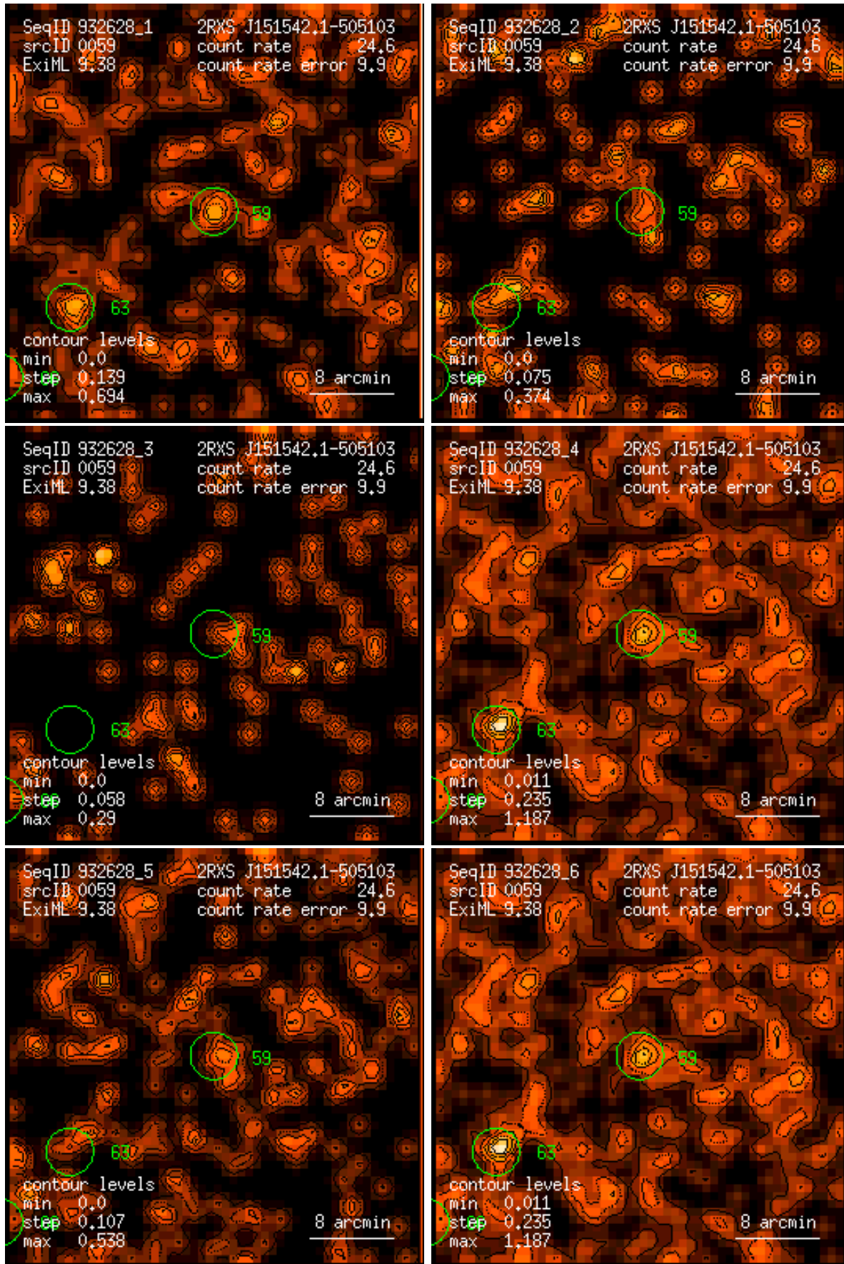
Figure 59: RASS 932628: detection 0059: band rate images, Gaussian filter: (1) PSPC channels 11 – 41, (2) 52 – 90, (3) 91 – 201, (4) 11 – 235, (5) 52 – 201, (6) 11 – 201. Broad band rates in counts/ks. Band rate contour levels in counts/ks/arcmin 2 .
