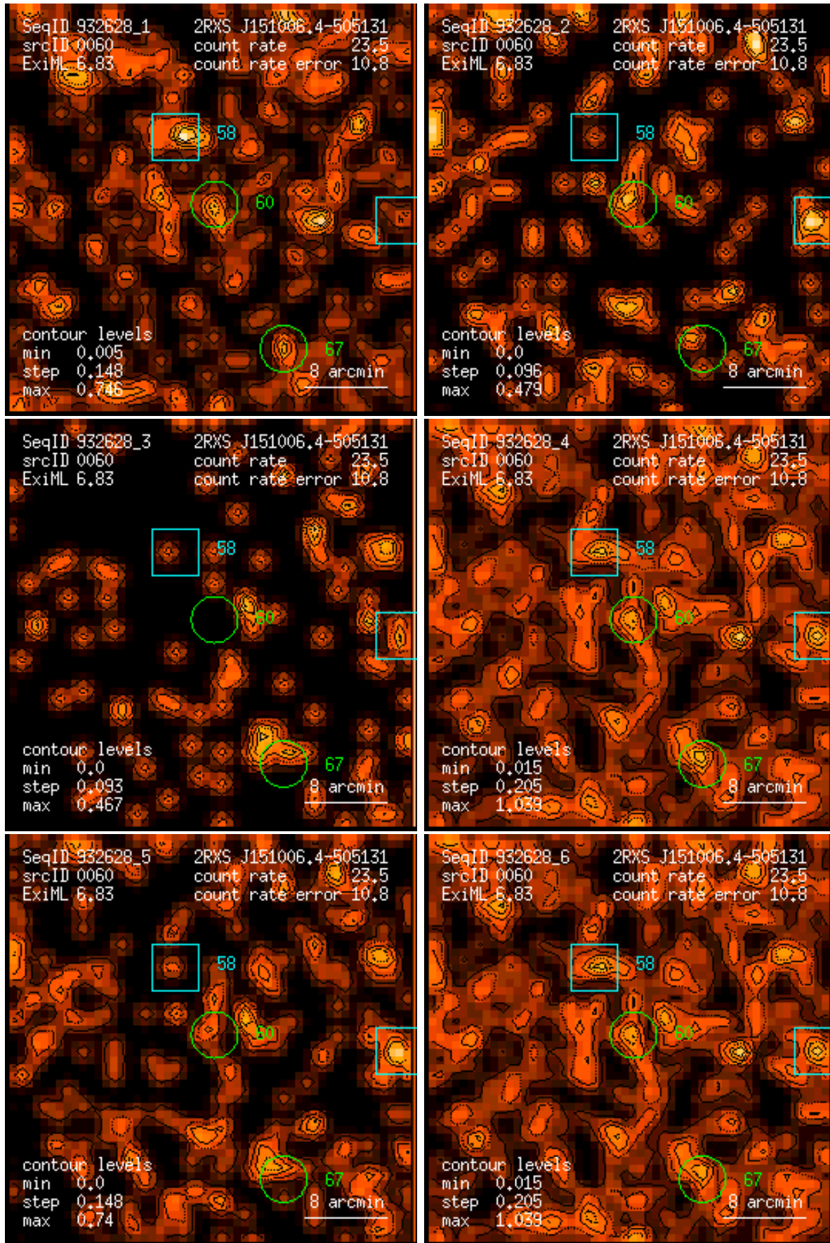
Figure 60: RASS 932628: detection 0060: band rate images, Gaussian filter: (1) PSPC channels 11 – 41, (2) 52 – 90, (3) 91 – 201, (4) 11 – 235, (5) 52 – 201, (6) 11 – 201. Broad band rates in counts/ks. Band rate contour levels in counts/ks/arcmin 2 .
