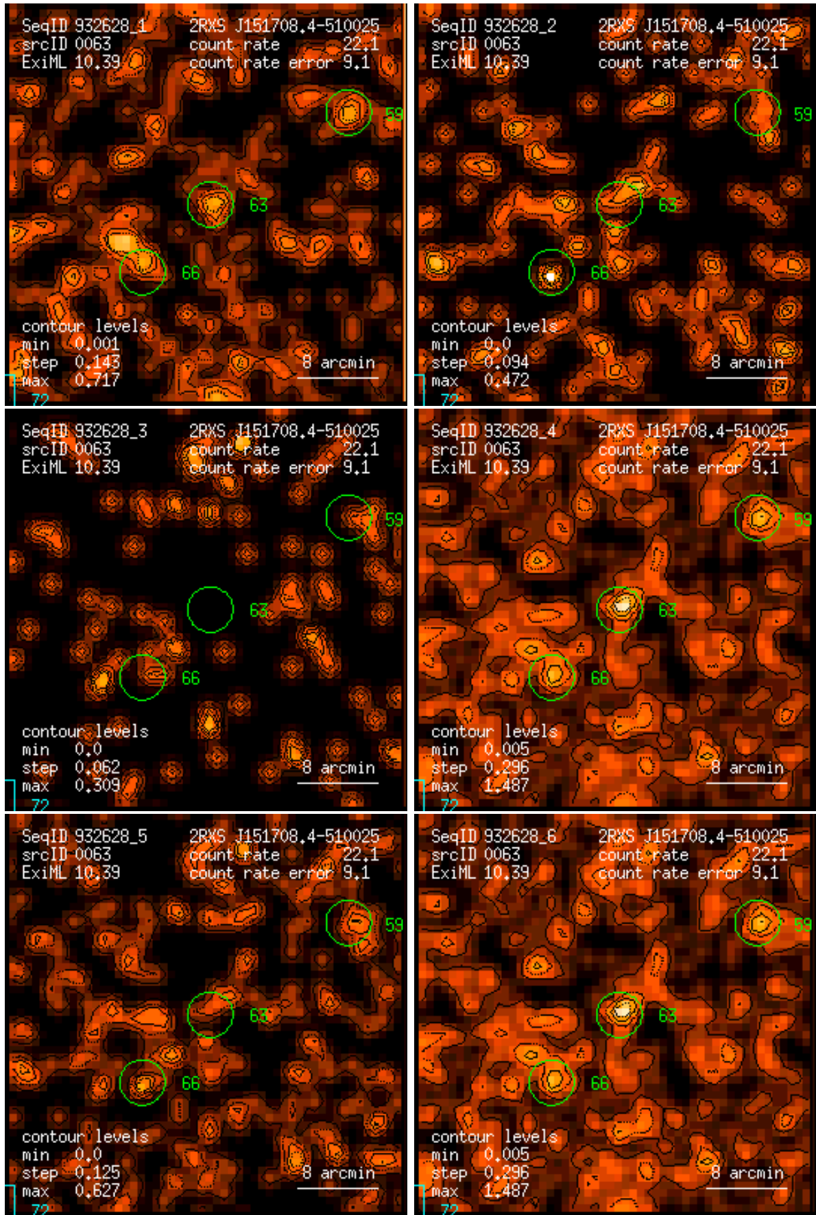
Figure 63: RASS 932628: detection 0063: band rate images, Gaussian filter: (1) PSPC channels 11 – 41, (2) 52 – 90, (3) 91 – 201, (4) 11 – 235, (5) 52 – 201, (6) 11 – 201. Broad band rates in counts/ks. Band rate contour levels in counts/ks/arcmin 2 .
