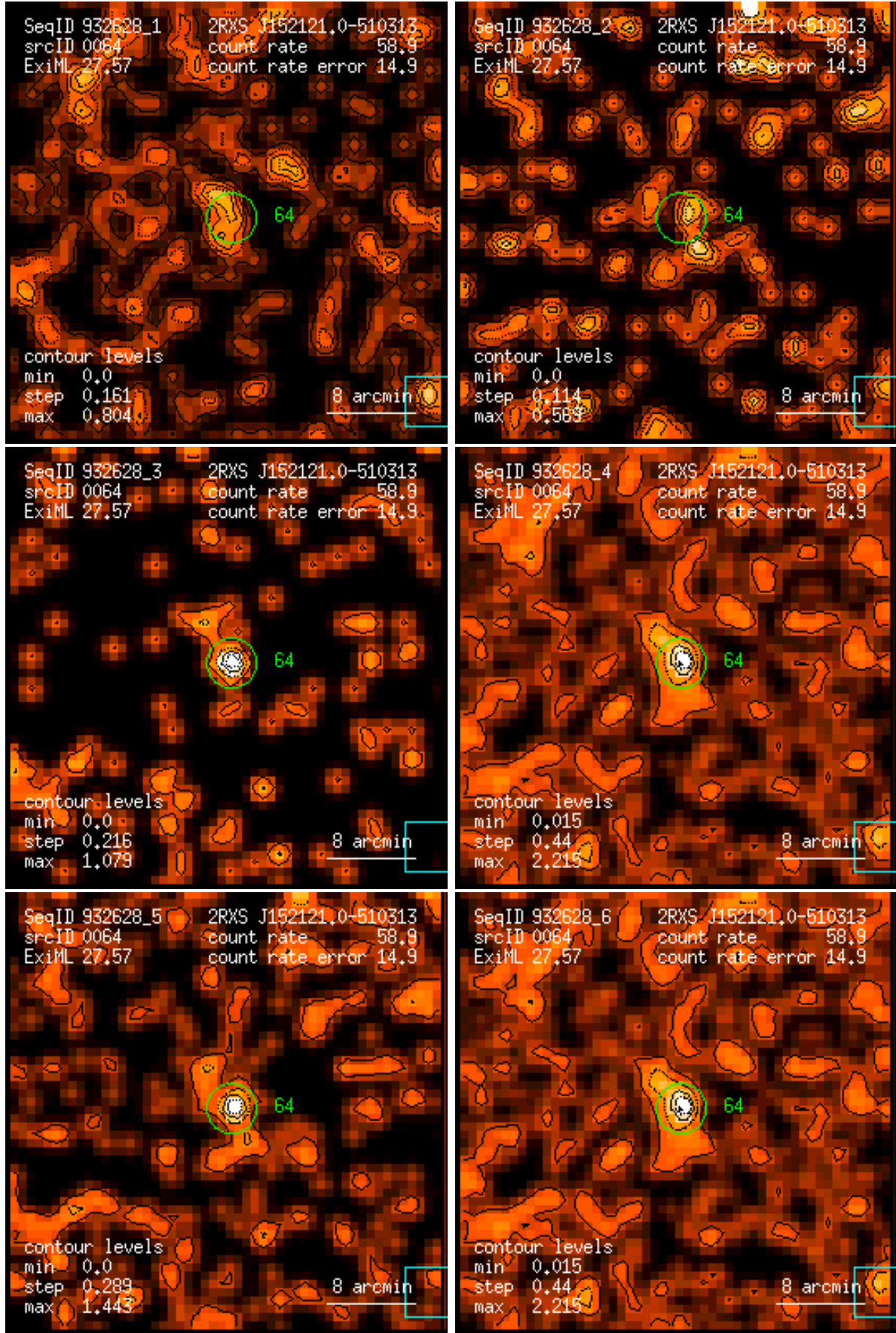
Figure 64: RASS 932628: detection 0064: band rate images, Gaussian filter: (1) PSPC channels 11 – 41, (2) 52 – 90, (3) 91 – 201, (4) 11 – 235, (5) 52 – 201, (6) 11 – 201. Broad band rates in counts/ks. Band rate contour levels in counts/ks/arcmin 2 .
