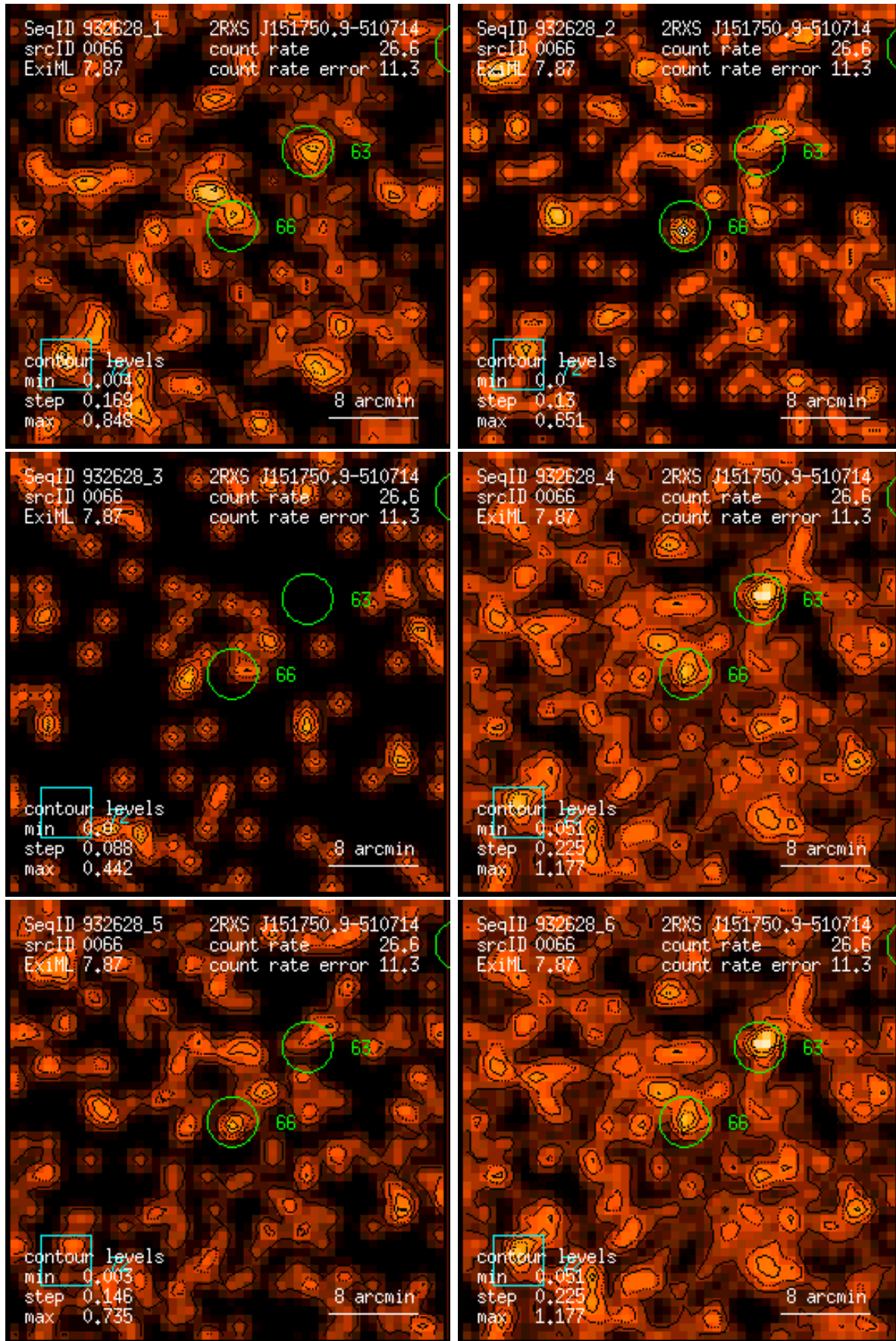
Figure 66: RASS 932628: detection 0066: band rate images, Gaussian filter: (1) PSPC channels 11 – 41, (2) 52 – 90, (3) 91 – 201, (4) 11 – 235, (5) 52 – 201, (6) 11 – 201. Broad band rates in counts/ks. Band rate contour levels in counts/ks/arcmin 2 .
