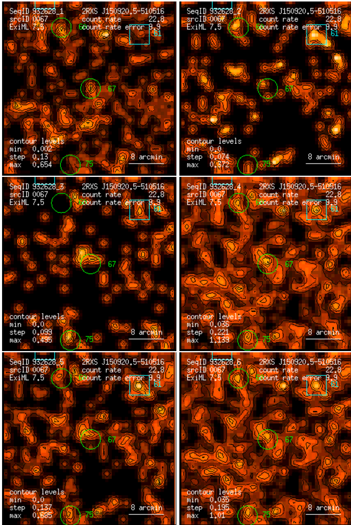
Figure 67: RASS 932628: detection 0067: band rate images, Gaussian filter: (1) PSPC channels 11 – 41, (2) 52 – 90, (3) 91 – 201, (4) 11 – 235, (5) 52 – 201, (6) 11 – 201. Broad band rates in counts/ks. Band rate contour levels in counts/ks/arcmin 2 .
