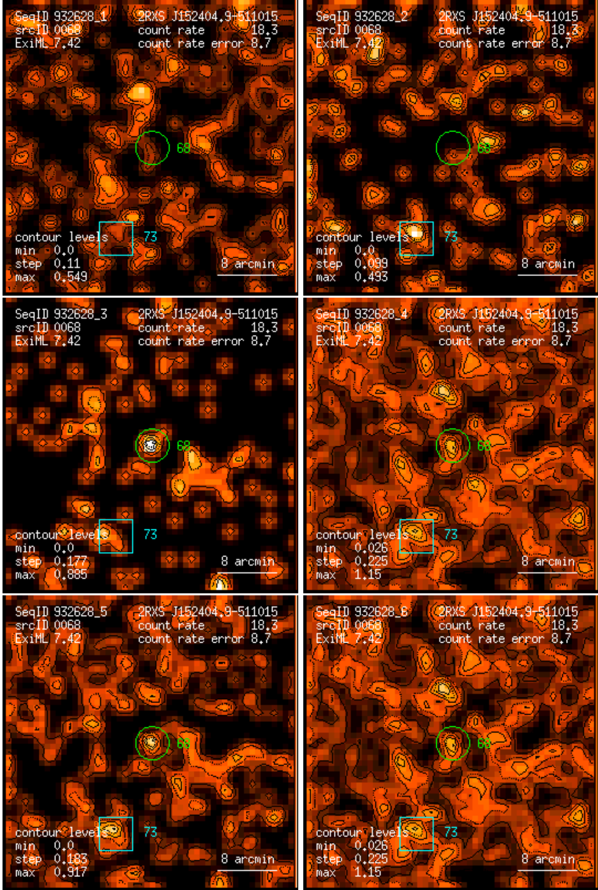
Figure 68: RASS 932628: detection 0068: band rate images, Gaussian filter: (1) PSPC channels 11 – 41, (2) 52 – 90, (3) 91 – 201, (4) 11 – 235, (5) 52 – 201, (6) 11 – 201. Broad band rates in counts/ks. Band rate contour levels in counts/ks/arcmin 2 .
